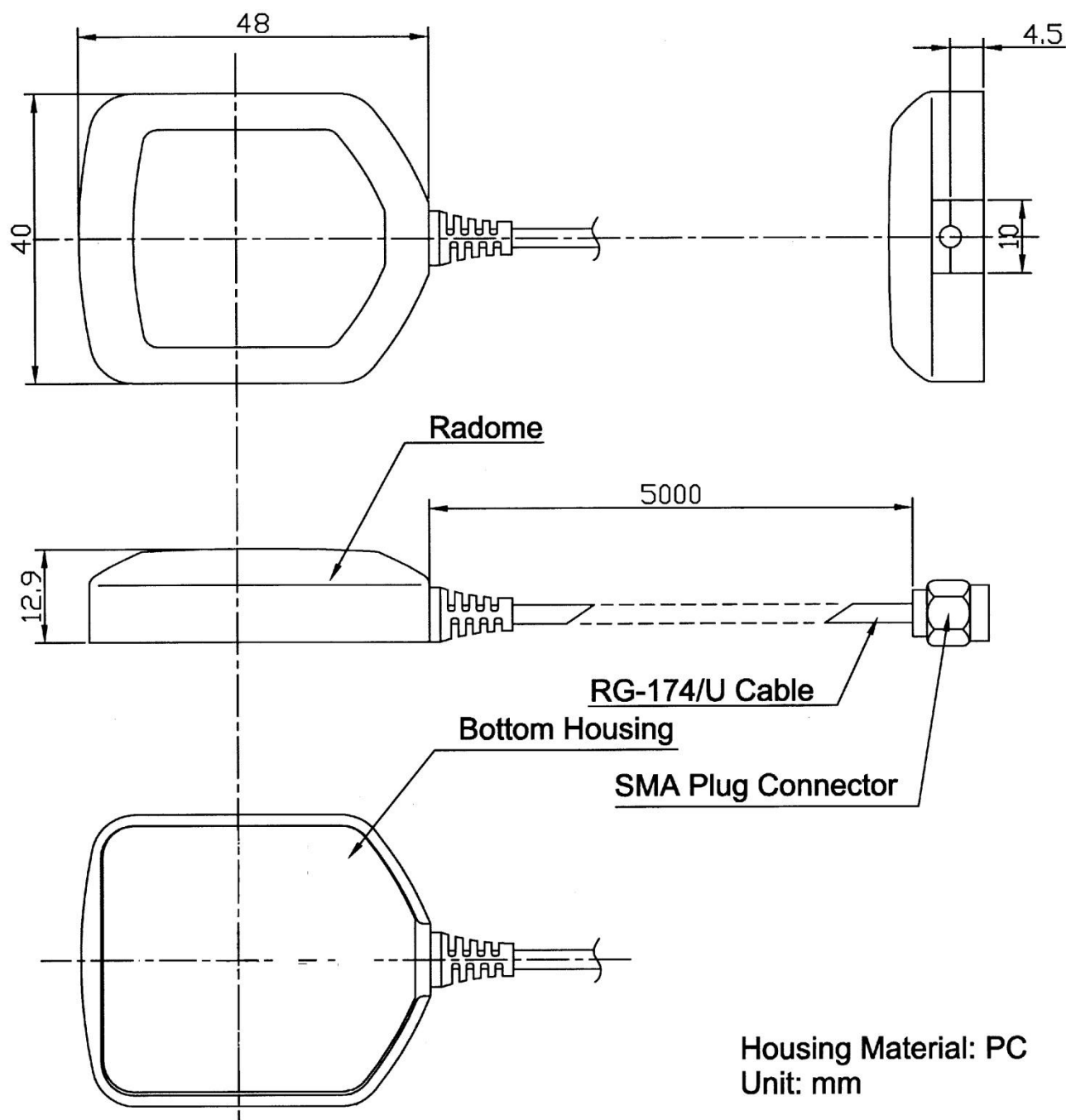
Figure 1: Mechanical outline
