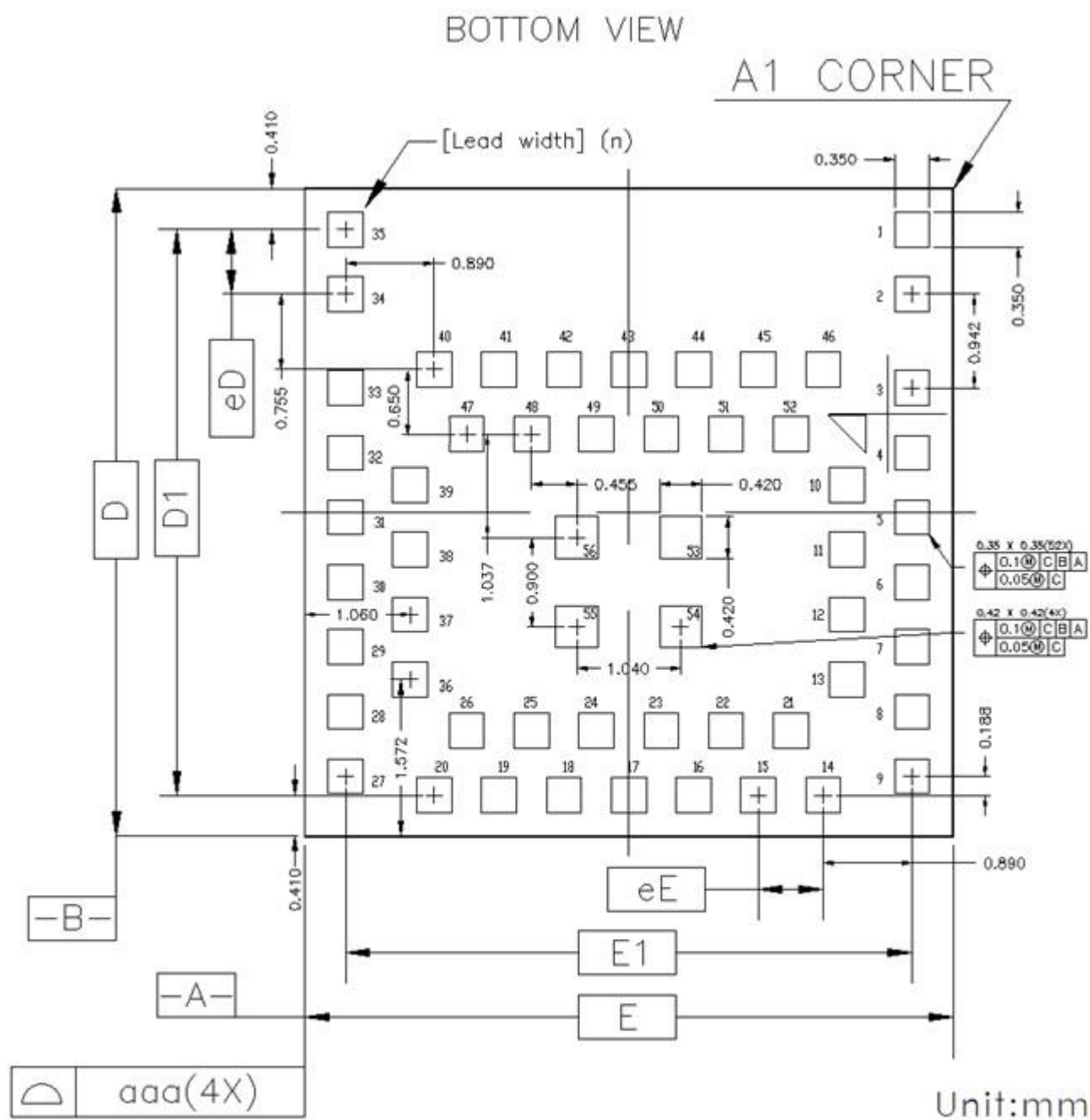
Figure 5: ANNA-B412 physical package outline – bottom view
