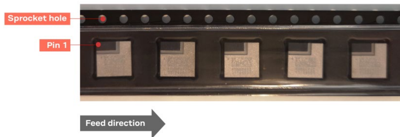
Figure 7: Orientation of ANNA-B4 modules on tape
