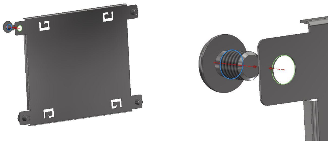
Figure 1. Mounting frame
