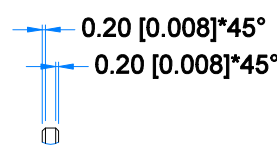
DETAIL C SCALE 4:1
