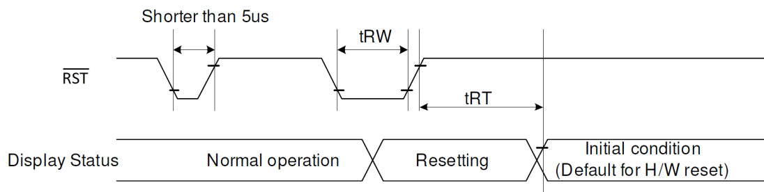
Figure 4: Reset Timing Diagram
