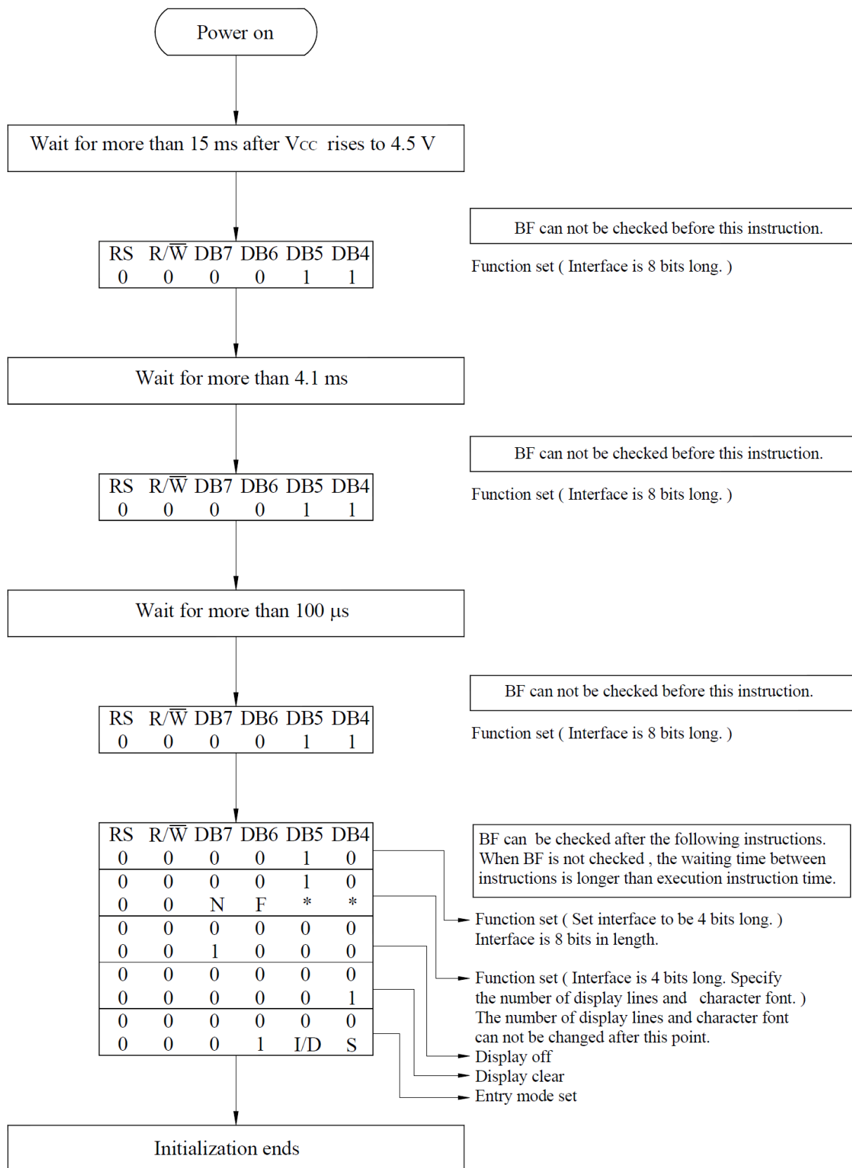
4-Bit Ineterface
