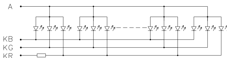
CIRCUIT DIAGRAM
