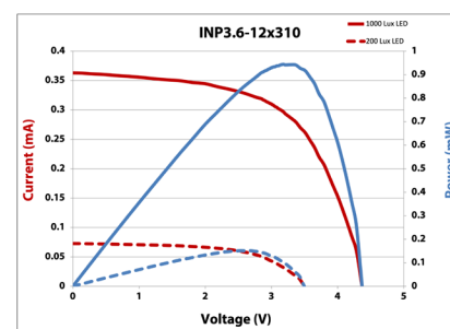
IV Curve
