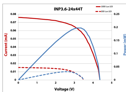
IV Curve
