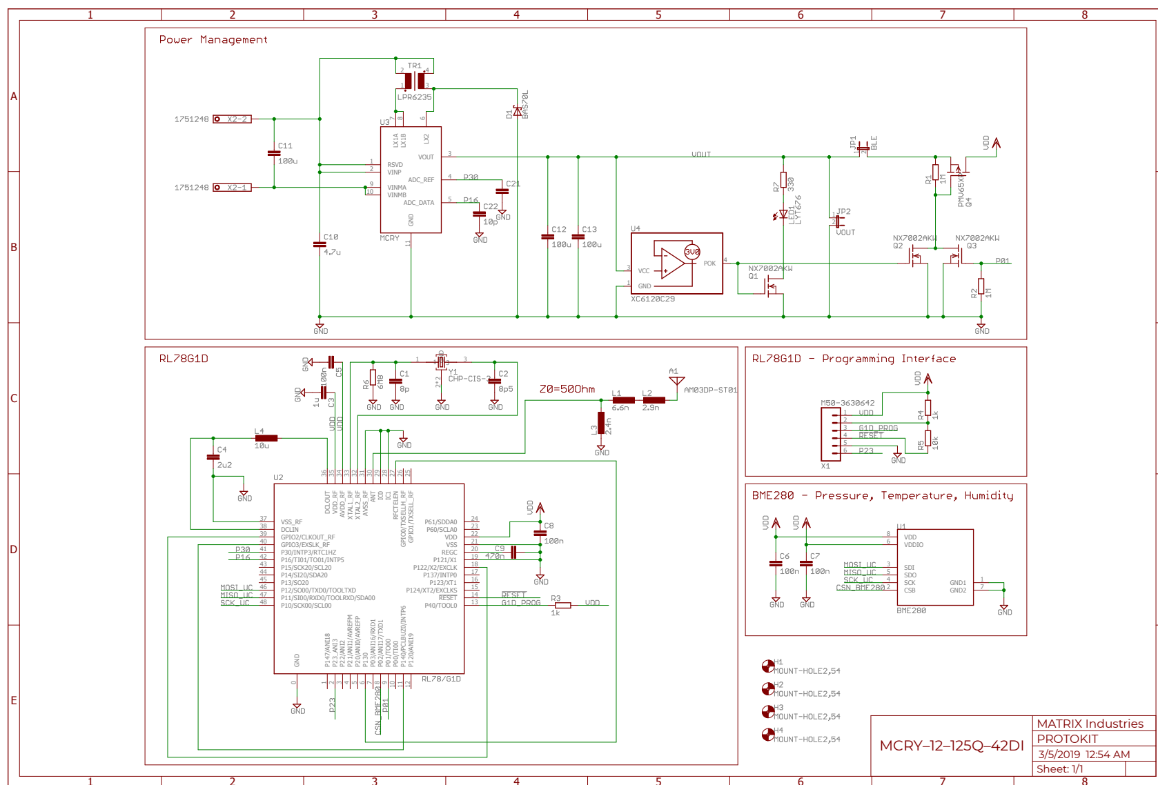
Figure 6: MCRY-PROTOKIT Schematics
