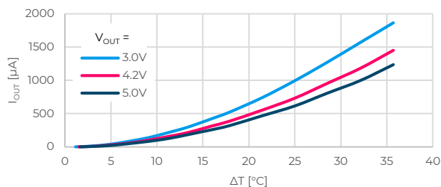
Figure 5. Output current for PRMT11-18305-** with 1/K_{TEC}=11\text{K/W}
