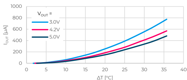
Figure 7. Output current for PRMT37-18305-** with 1/K_{TEC}=37\text{K/W}
