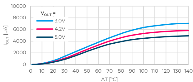
Figure 9. Output current for PRMT11-18305-**A with 1/K_{TEC}=11\text{K/W}
