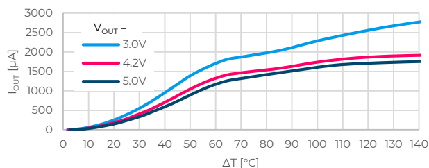
Figure 11. Output current for PRMT37-18305-**A with 1/K_{TEC}=37\text{K/W}
