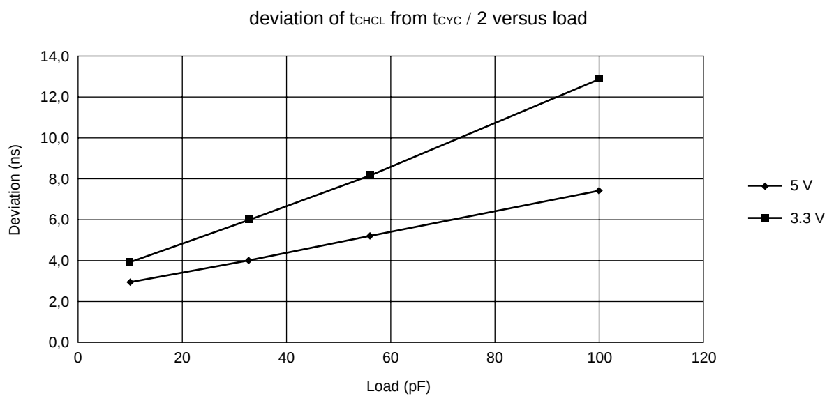
Deviation of t_{CHCL} from t_{CYC} / 2 versus load (Odd CLKB/CLKT division ratios) :
