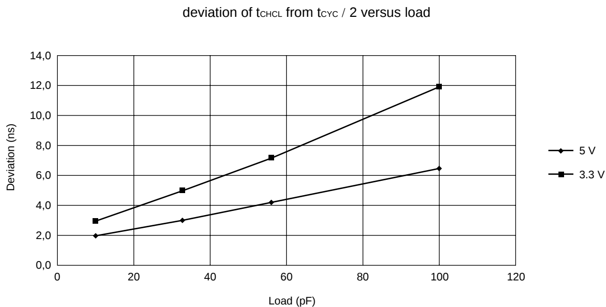
Deviation of t_{CHCL} from t_{CYC} / 2 versus load (Even CLKB/CLKT division ratios) :
