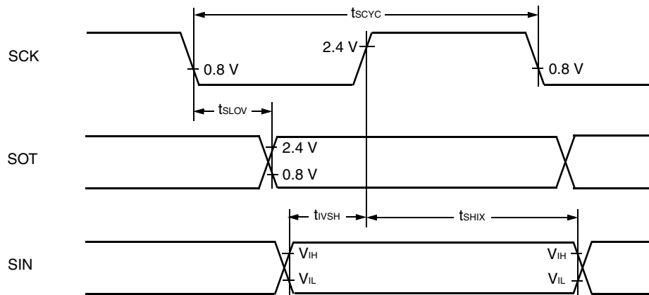
Internal Shift Clock Mode
