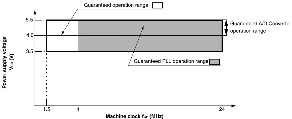
Guaranteed operation range of MB90860E series
