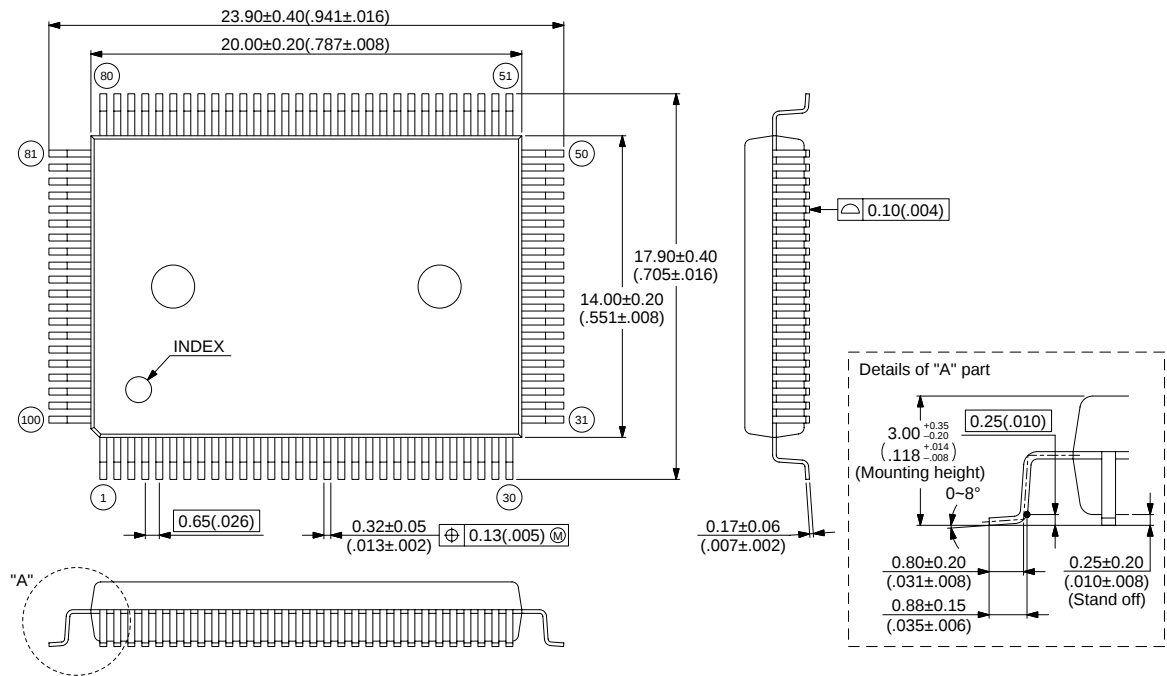
100-pin plastic QFP (FPT-100P-M06)
