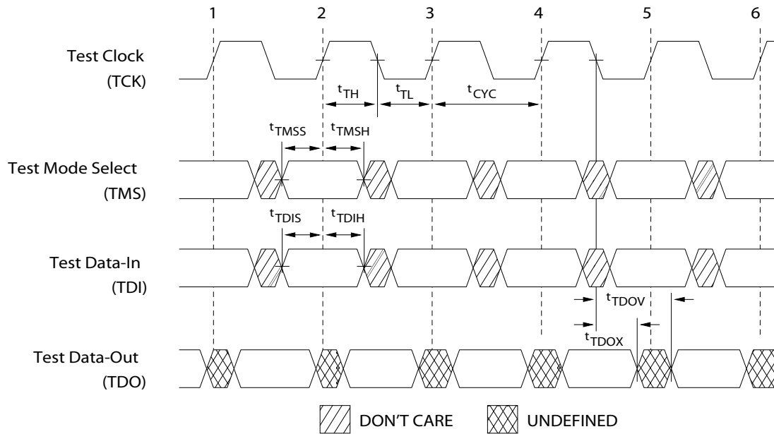
Figure 3. TAP Timing
