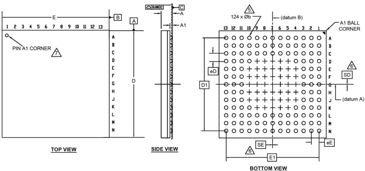
Figure 4. 124-BGA 9.0 × 9.0 × 1.0 mm
