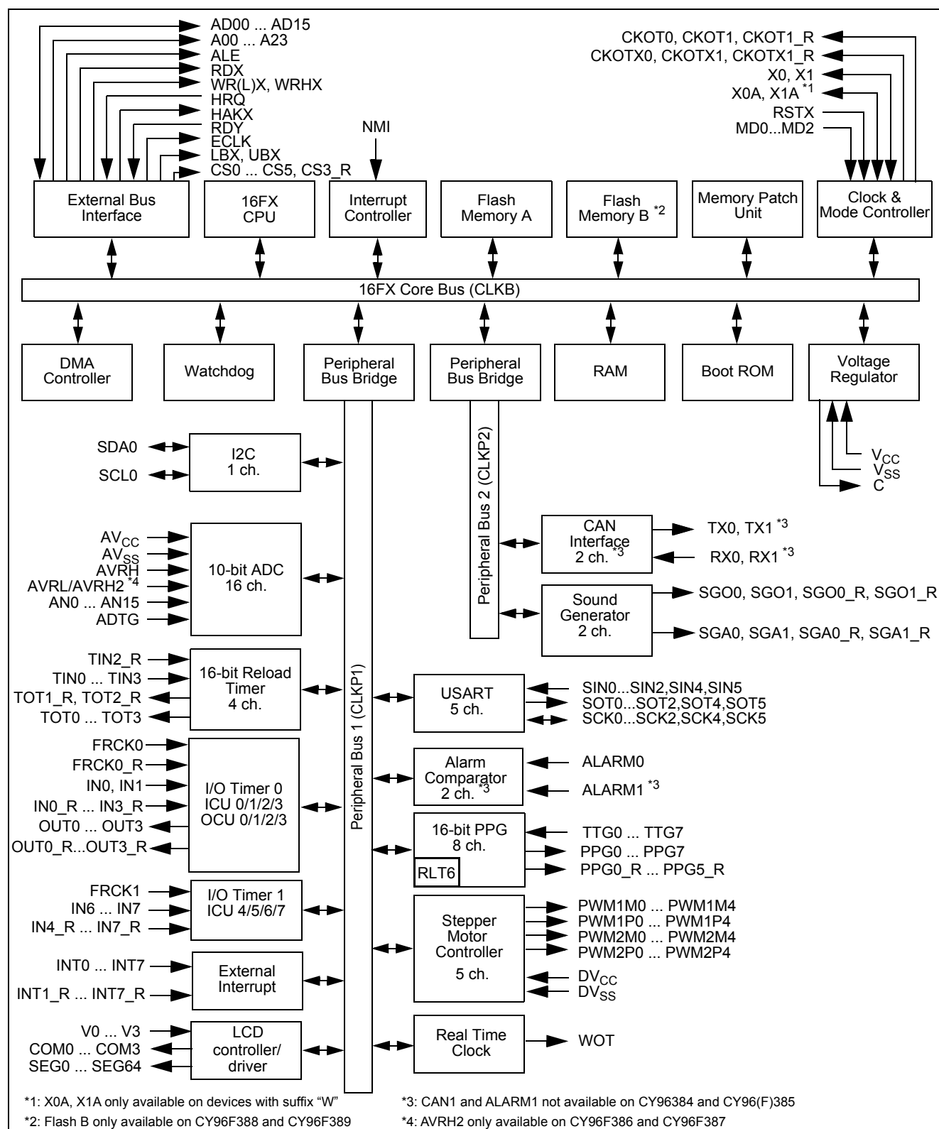
Block diagram of CY96(F)38x
