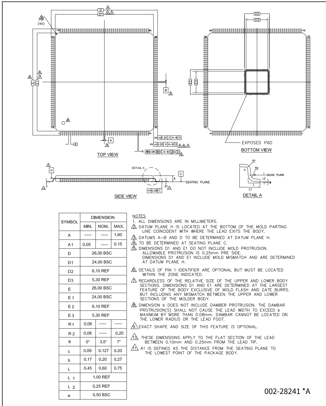
Figure 28-3 Package outline – 176-TQFP
