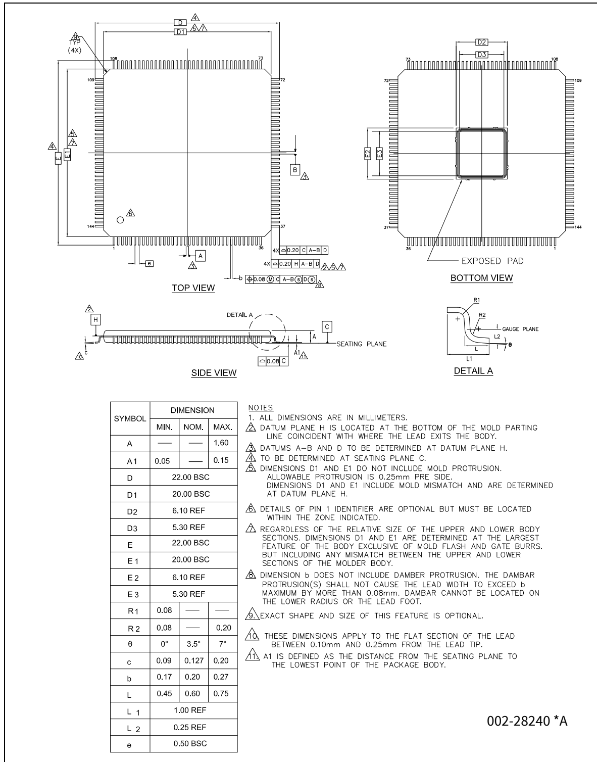
Figure 28-2 Package outline - 144-TQFP
