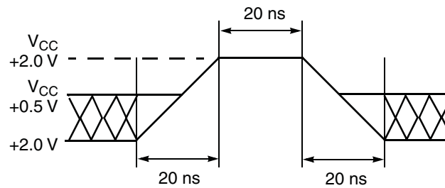
Figure 12.4 Maximum Positive Overshoot Waveform
