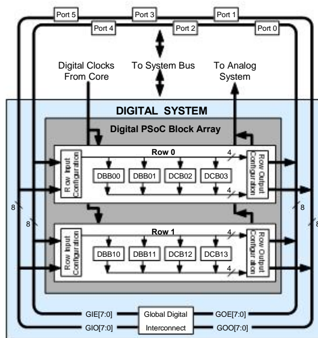
Figure 1-1. Digital System Block Diagram
