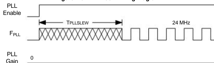
Figure 7-3. PLL Lock Timing Diagram
