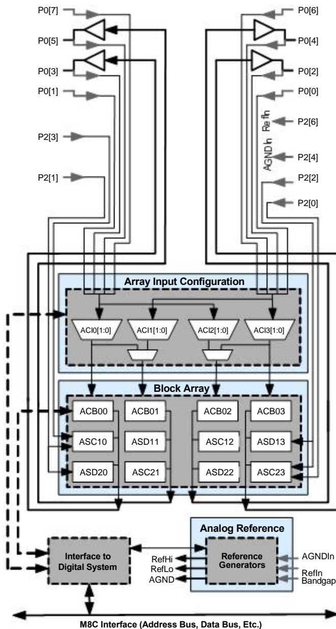
Figure 1-2. Analog System Block Diagram
