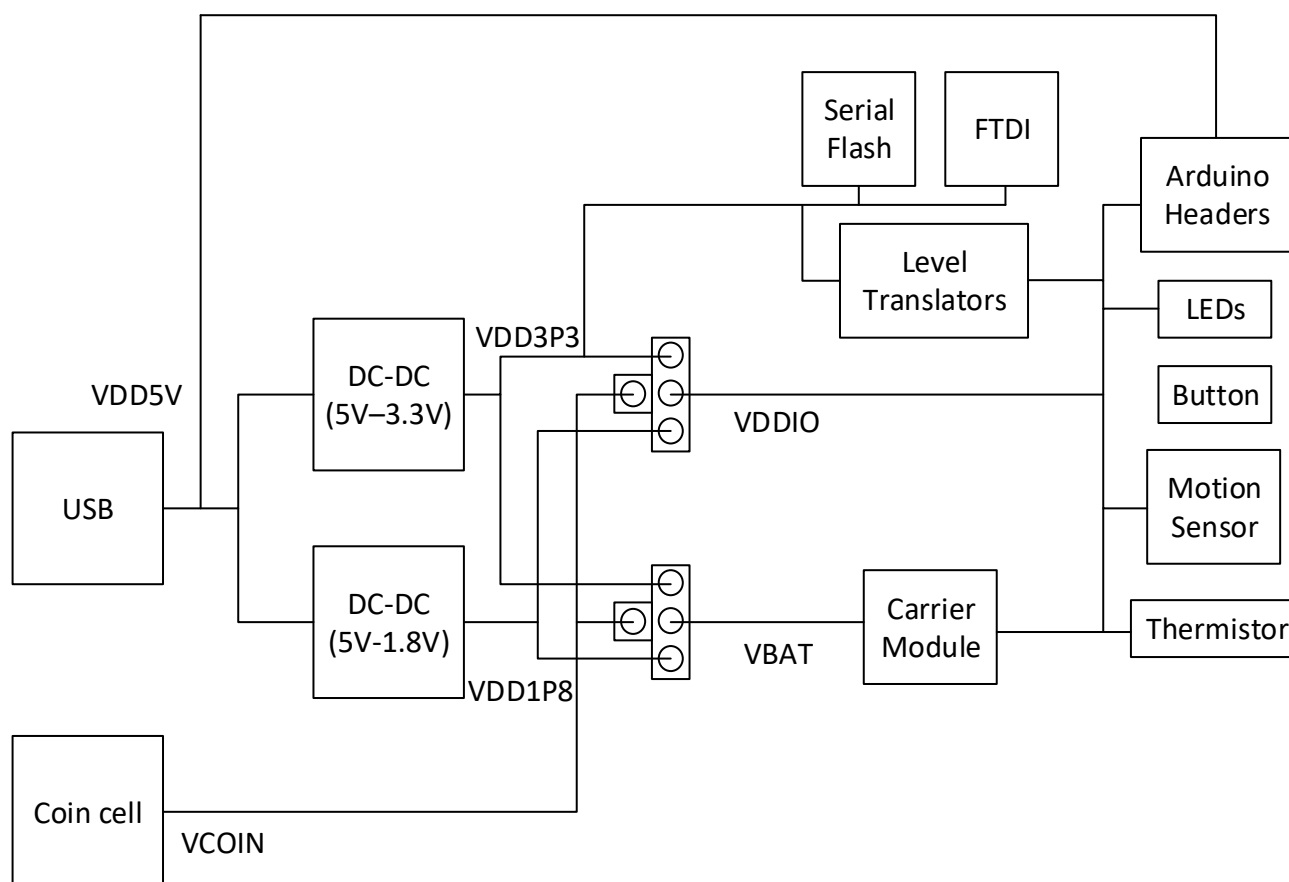
Figure 5-1. Power Architecture
