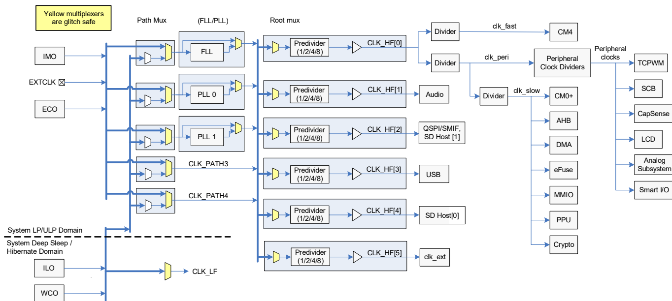
Figure 3. Clocking Diagram
