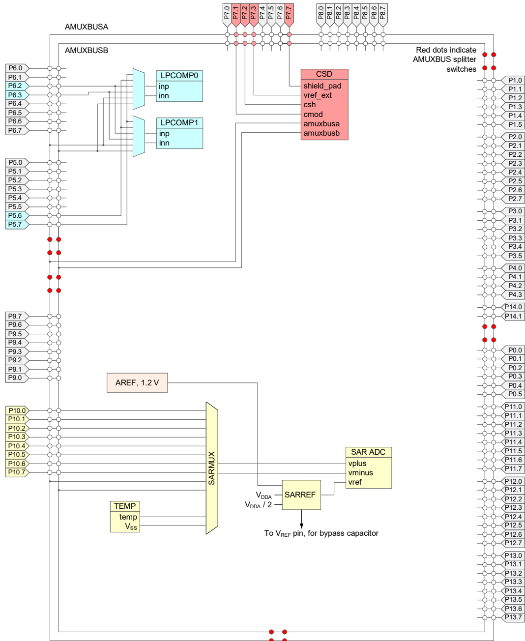
Figure 6. Analog Subsystem
