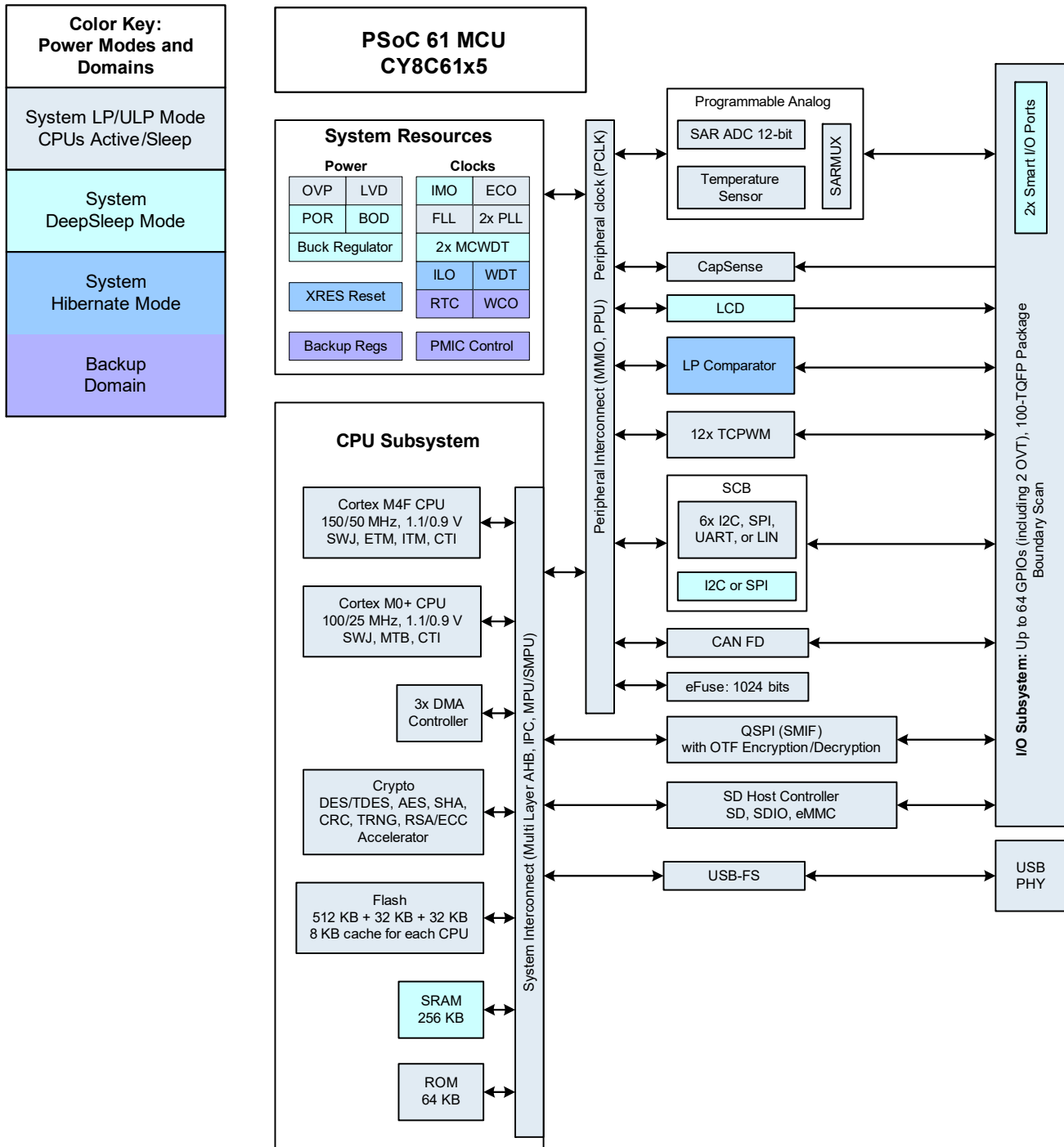
Figure 2. Block Diagram
