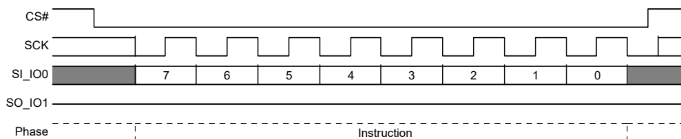
Figure 59. Enter QPI Mode (QPIEN 38h) Command Sequence
