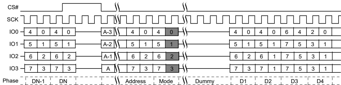
Figure 69. Continuous Quad I/O Read Command Sequence [32, 33]
