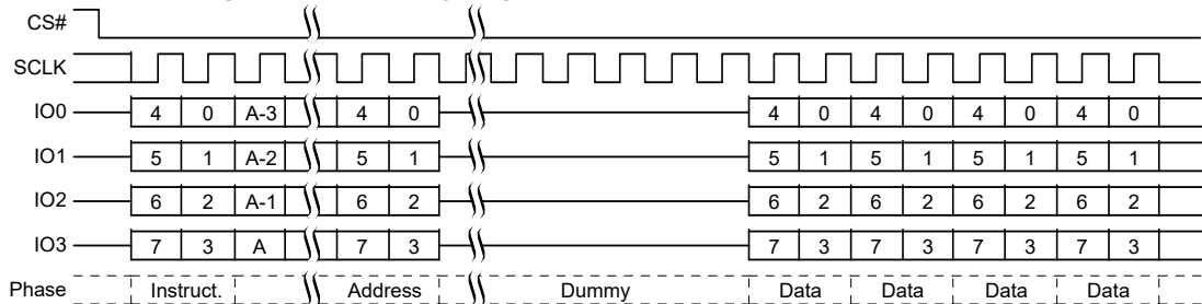
Figure 56. Read Any Register, QPI Mode, Command Sequence [25]
