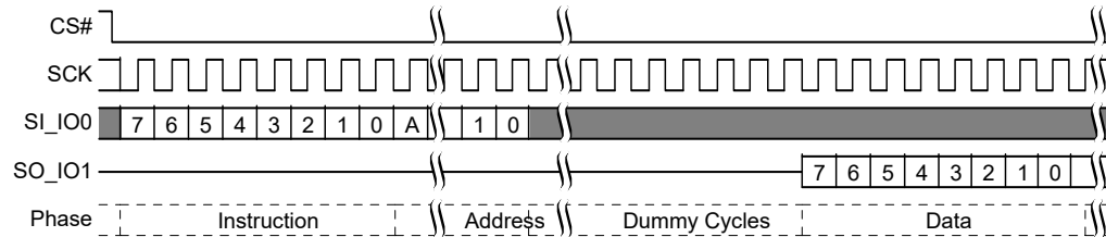
Figure 55. Read Any Register Read Command Sequence [25]
