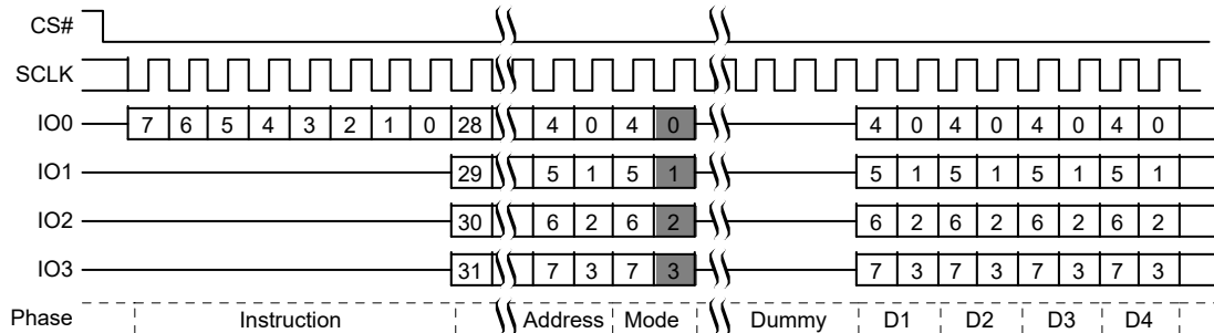
Figure 16. Quad I/O Command [3]
