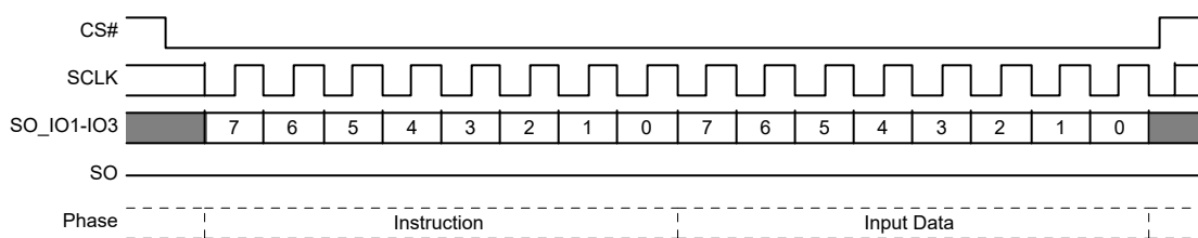
Figure 10. Single Bit Wide Input Command
