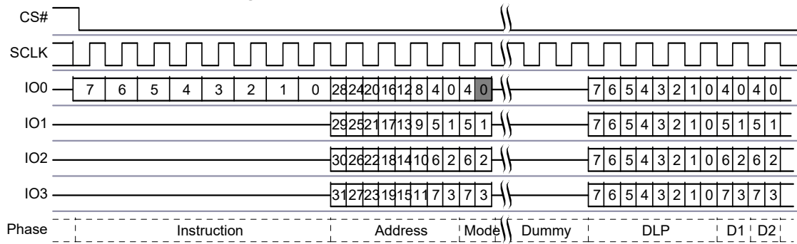
Figure 18. DDR Quad I/O Read Command [4]
