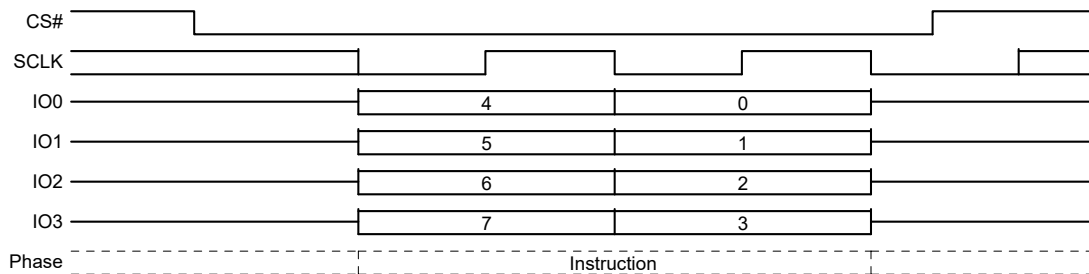
Figure 85. Program or Erase Suspend Command Sequence QPI mode
