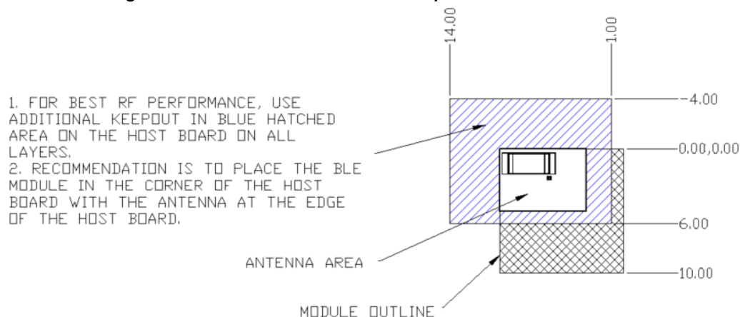
Figure 3. Recommended Host PCB Keep Out Area Around the CYBLE-022001-00 Chip Antenna
