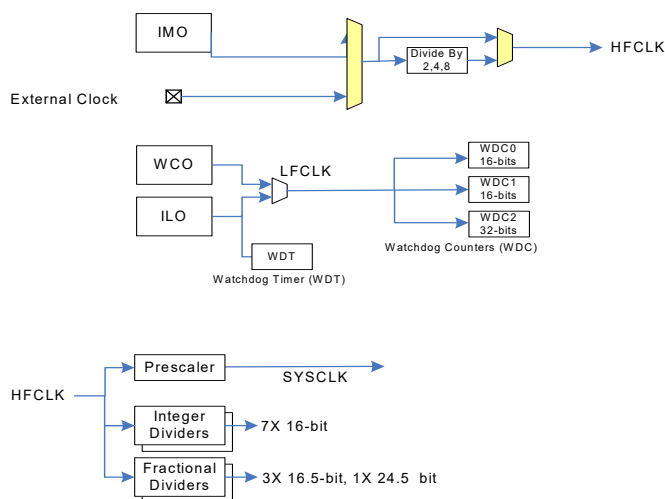
Figure 3. PSoC 4100PS MCU Clocking Architecture
