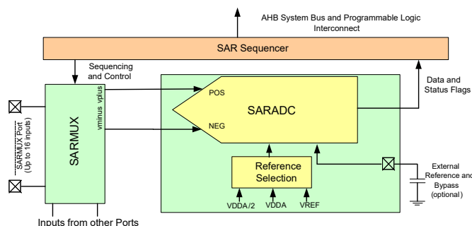
Figure 5. SAR ADC
