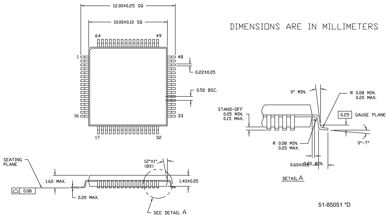
Figure 9. 64-pin TQFP Package (0.5-mm Pitch) Outline
