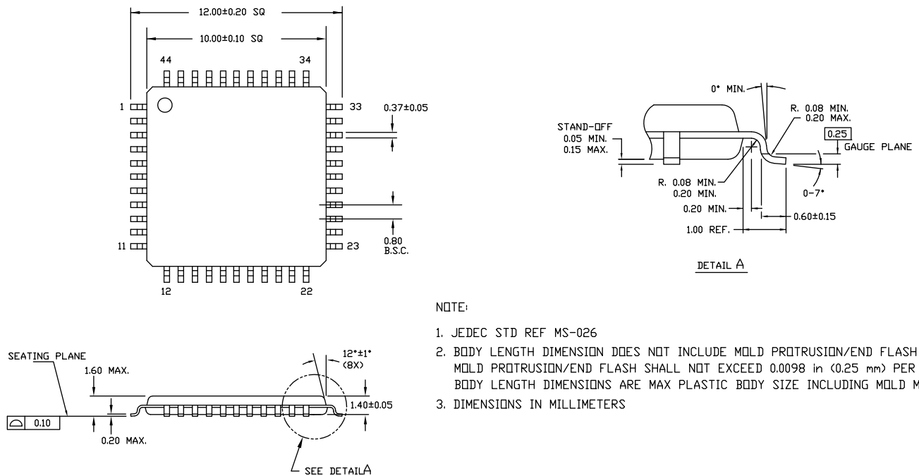
Figure 10. 44-Pin TQFP Package Outline
