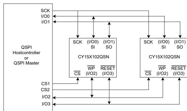
Figure 3. System Configuration with QSPI Port
