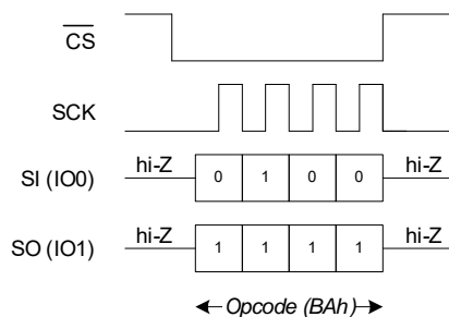
Figure 104. Hibernate Mode Operation in DPI Mode
