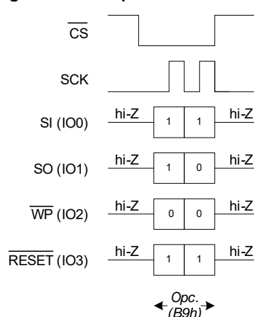
Figure 101. Deep Power-Down Mode Operation in QPI Mode
