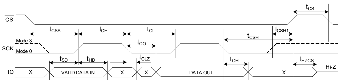
Figure 115. SPI Switching Timing - Multiple I/O, SDR (Mode 0 and Mode 3)
