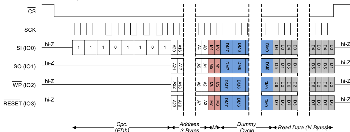
Figure 64. Quad I/O Read in DDR (DDRQIOR) – In Extended SPI Mode
