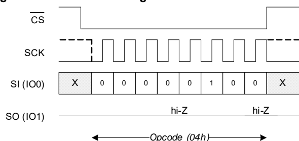
Figure 9. WRDI Bus Configuration in SPI Mode
