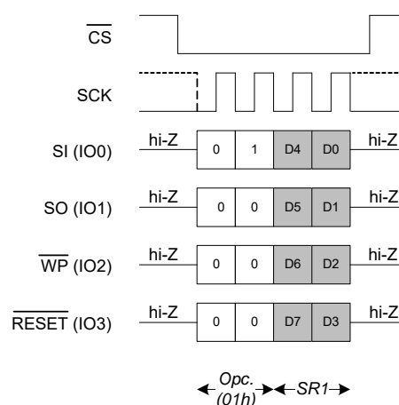
Figure 14. WRSR in QPI Mode (WREN not shown)
