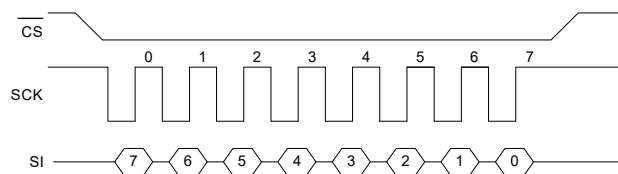
Figure 5. SPI Mode 3
