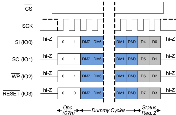
Figure 20. Read SR2 (RDSR2) in QPI Mode
