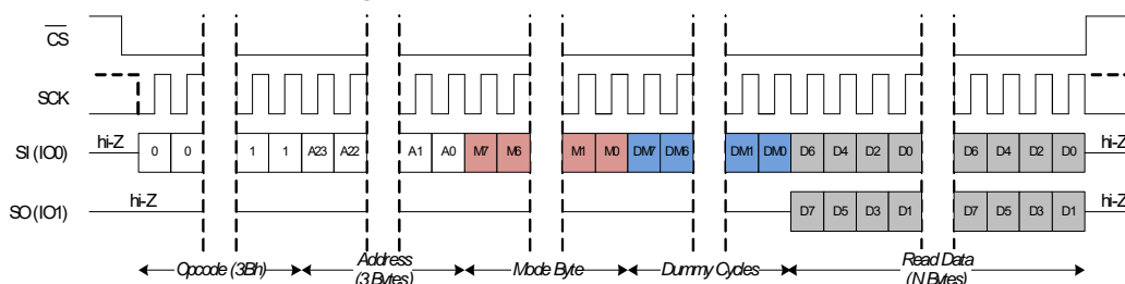
Figure 59. Double Output Read (DOR)
