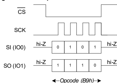
Figure 100. Deep Power-Down Mode Operation in DPI Mode
