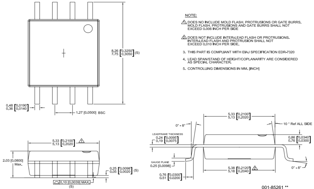
Figure 121. 8-pin SOIC (208 Mils) Package Outline, 001-85261
