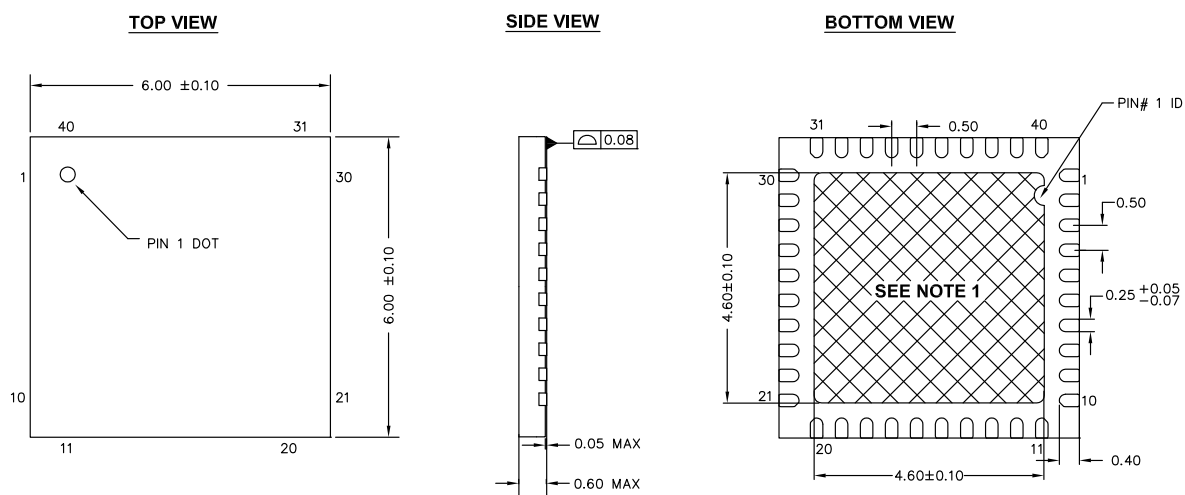
Figure 10. 40-Pin QFN (6 × 6 × 0.6 mm), LR40A/LQ40A 4.6 × 4.6 E-PAD (Sawn) Package Outline, 001-80659
