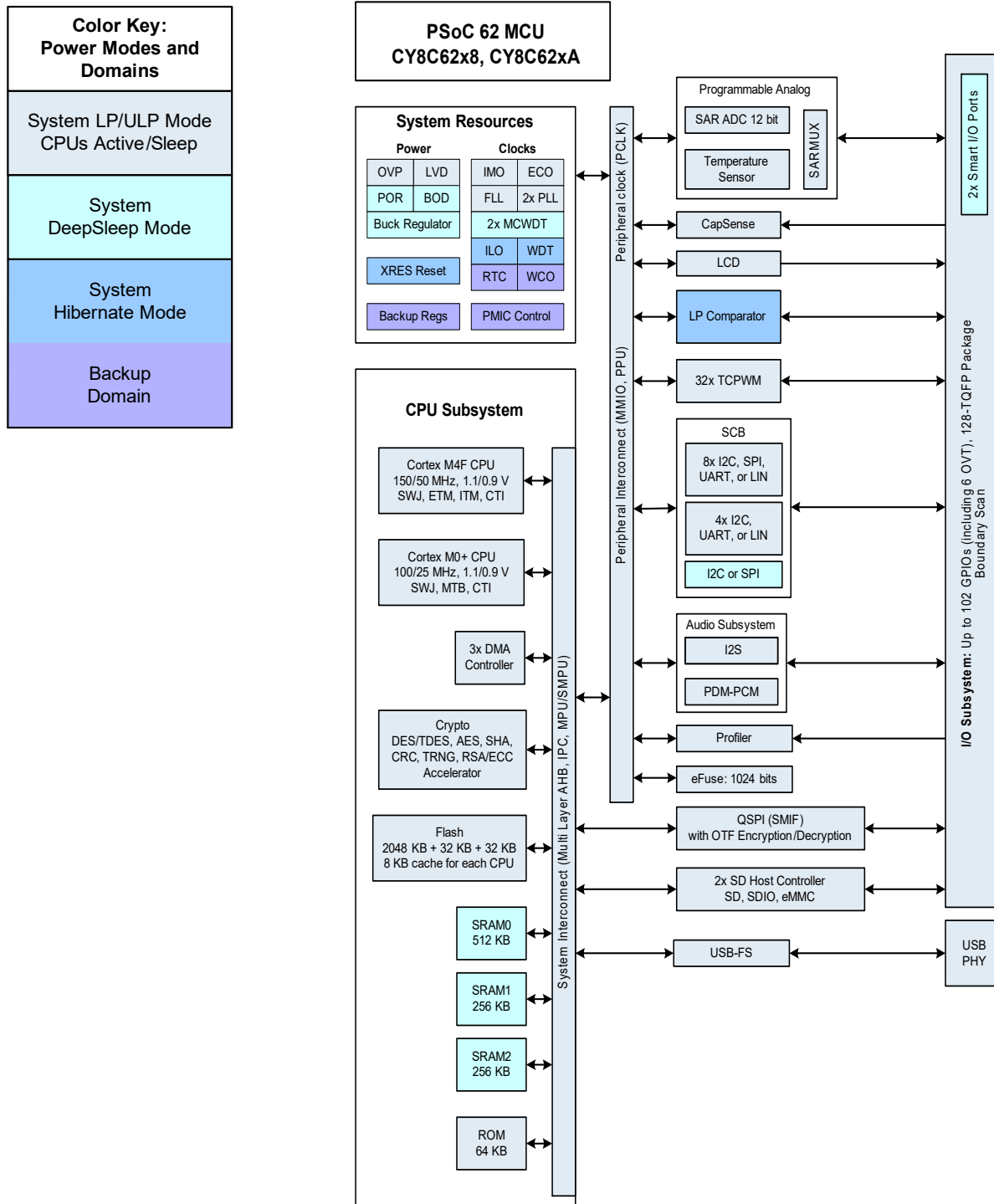
Figure 2. Block Diagram
