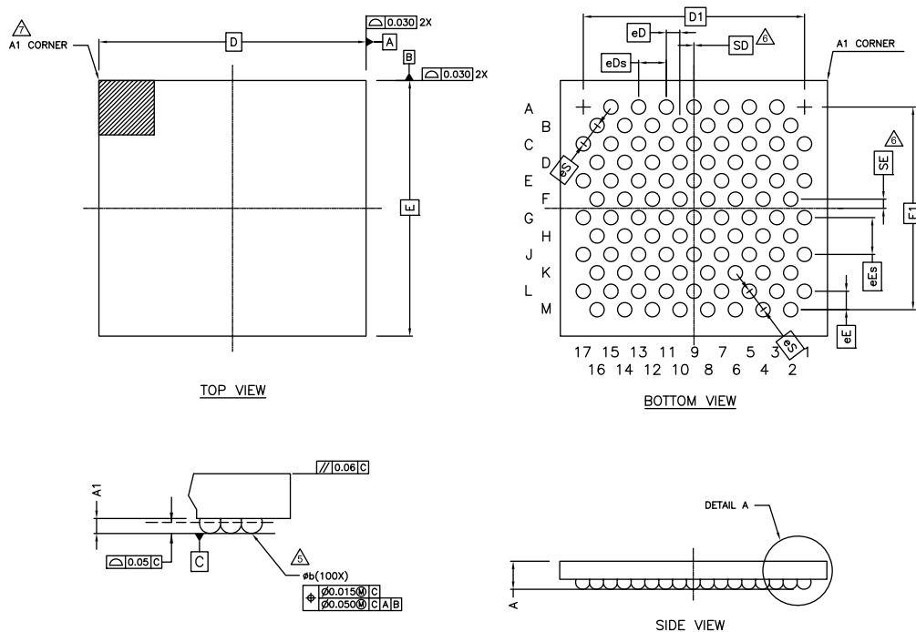
Figure 19. 100-WLCSP 4.1068 × 3.9025 × 0.467mm
