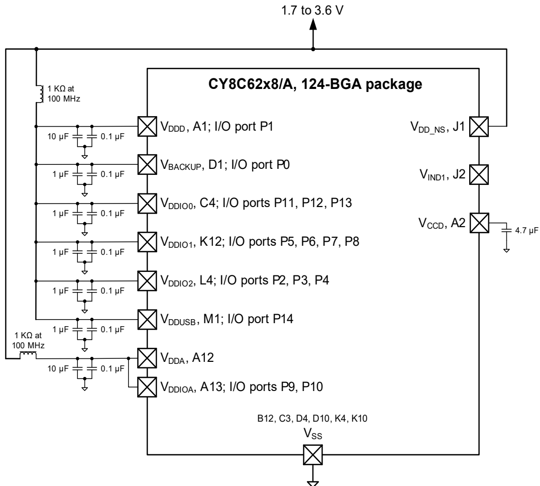
Figure 13. 124-BGA (No Buck) Power Connection Diagram
