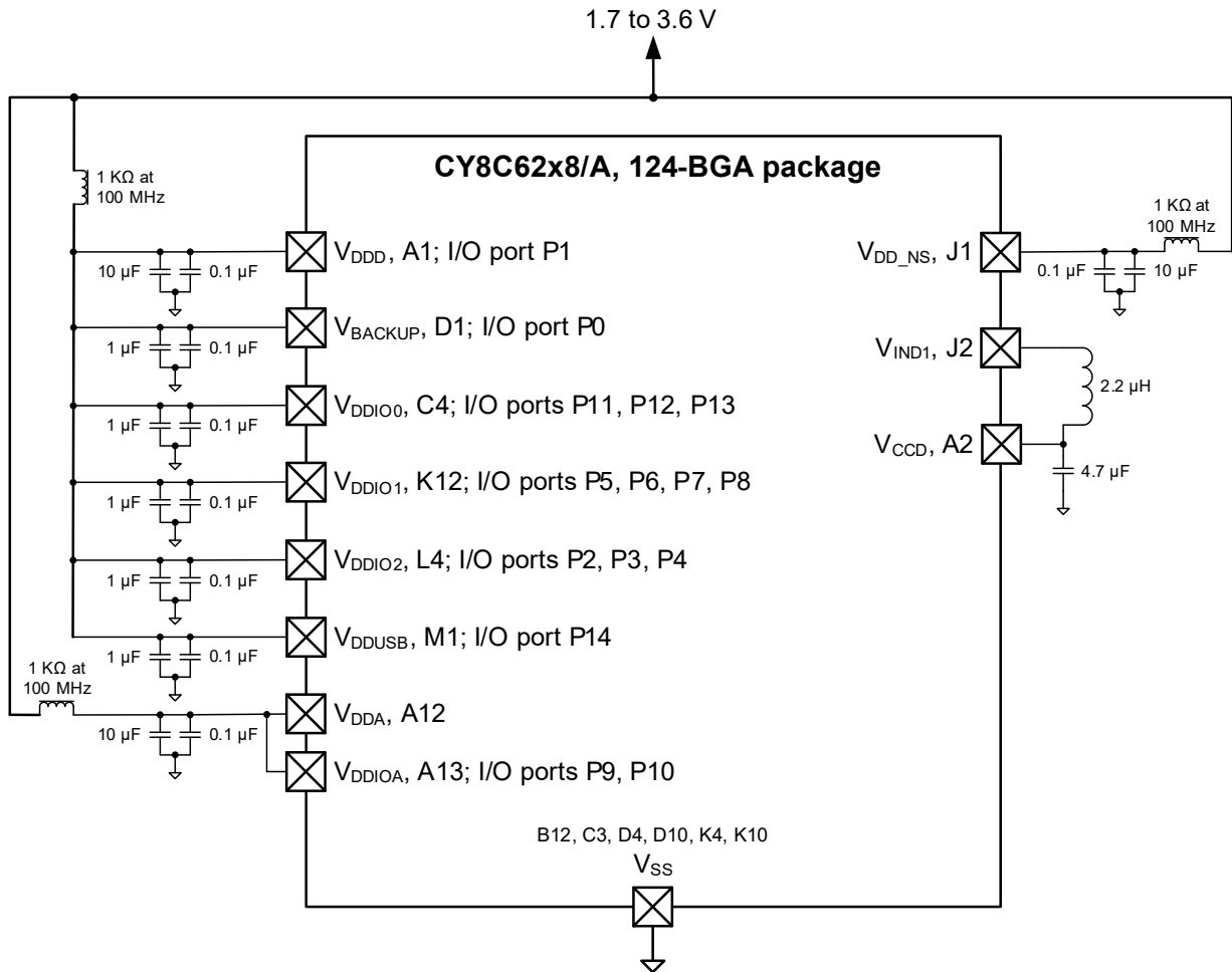
Figure 12. 124-BGA Power Connection Diagram
