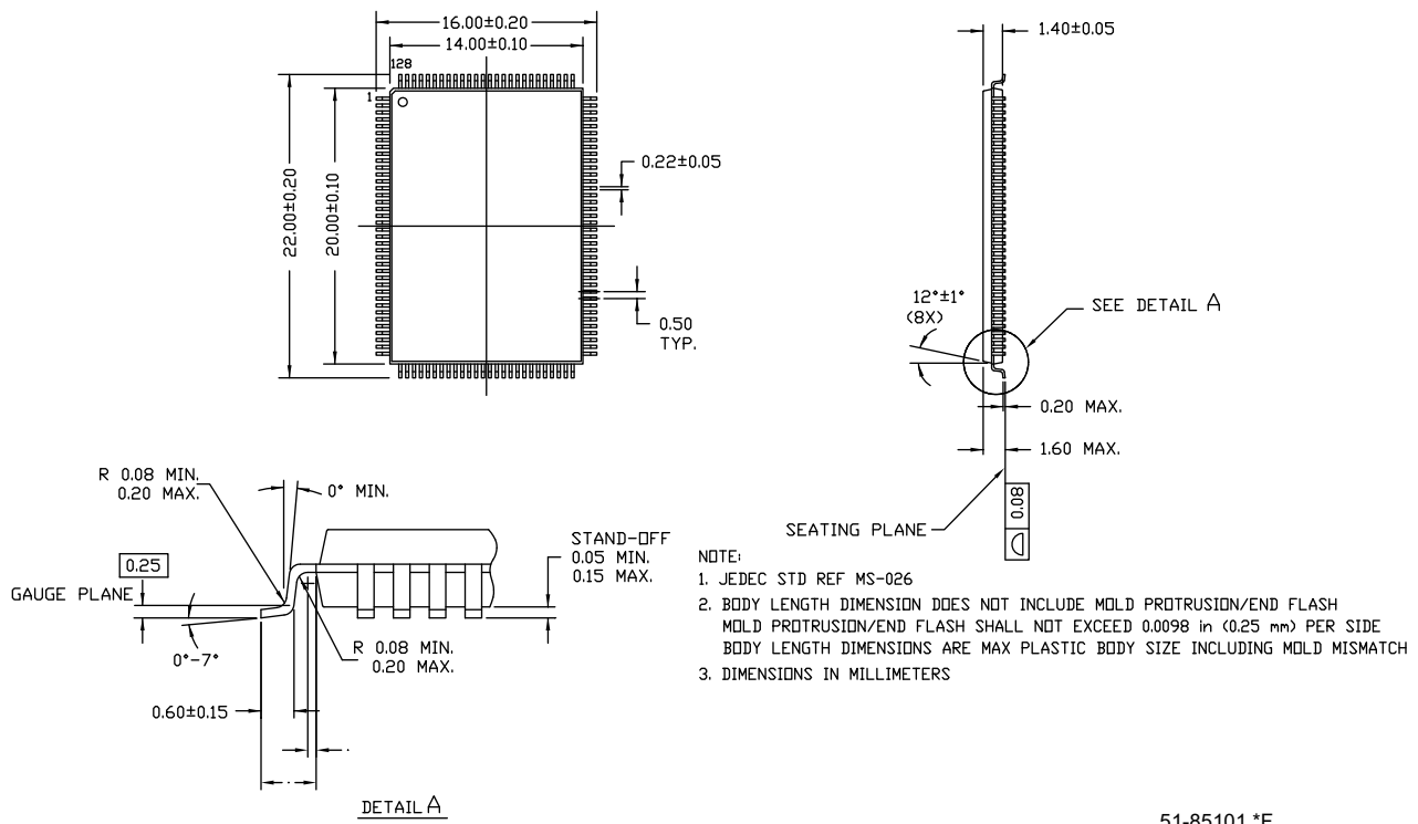
Figure 18. 128-TQFP 14.0 × 20.0 × 1.4 mm
