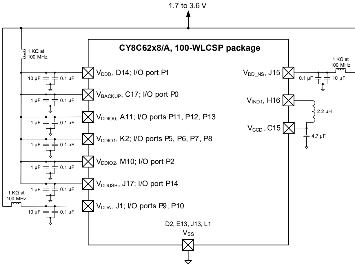
Figure 14. 100-WLCSP Power Connection Diagram
