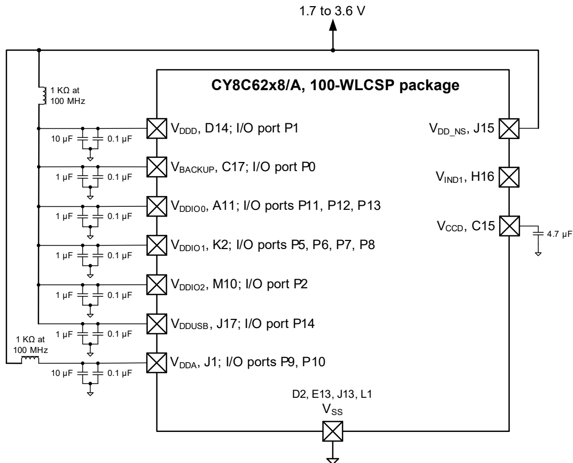
Figure 15. 100-WLCSP (No Buck) Power Connection Diagram
