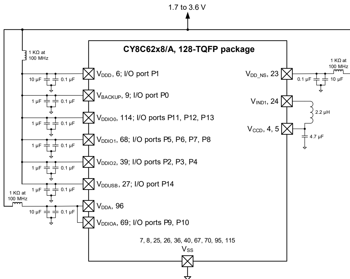
Figure 10. 128-TQFP Power Connection Diagram
