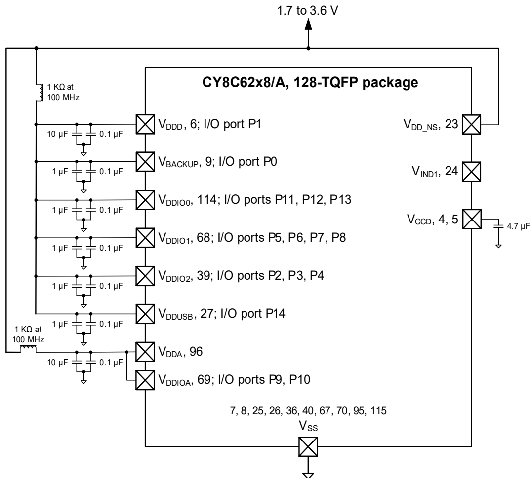
Figure 11. 128-TQFP (No Buck) Power Connection Diagram
