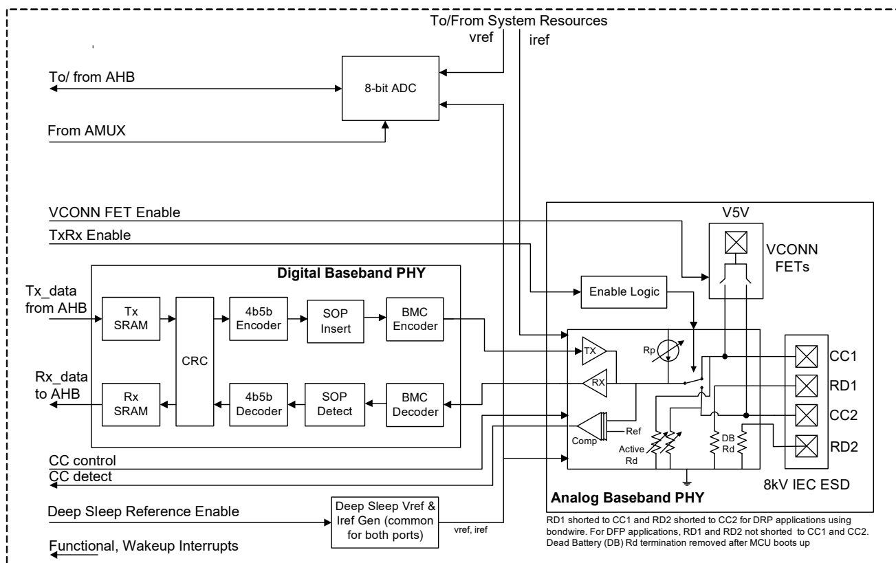
Figure 1. USB-PD Subsystem
