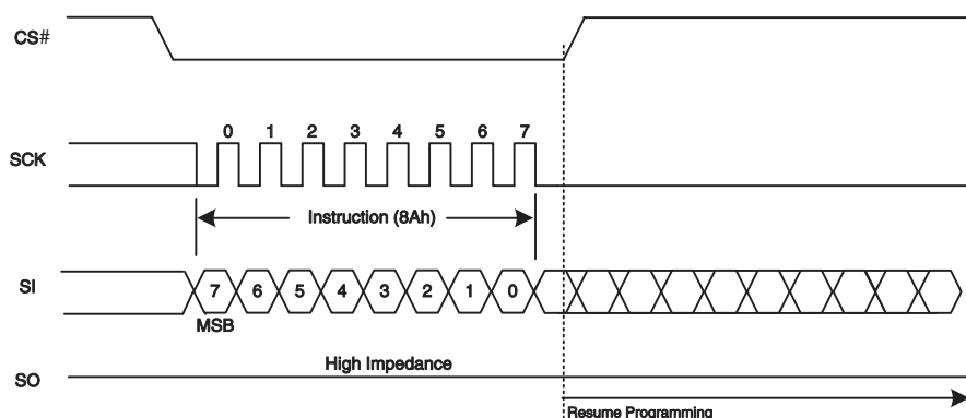
Figure 102 Program Resume Command Sequence
