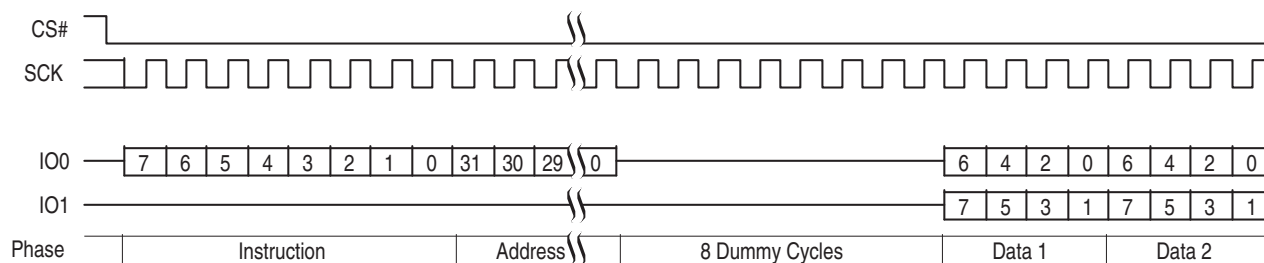
Figure 71 Dual Output Read Command Sequence (4-byte Address, 3Ch or 3Bh [ExtAdd=1, LC=11b])
