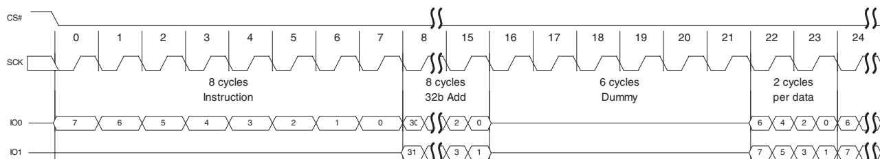
Figure 90 DDR Dual I/O Read (4-byte Address, BEh or BDh [ExtAdd=1], HPLC=00b)
