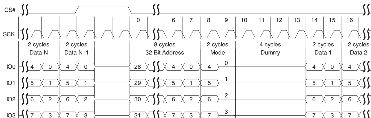
Figure 82 Continuous Quad I/O Read Command Sequence (4-byte Address), LC=00b
