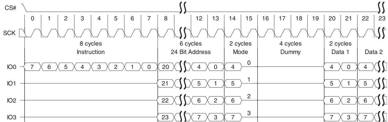
Figure 79 Quad I/O Read Command Sequence (3-byte Address, EBh [ExtAdd=0], LC=00b)
