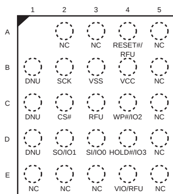
Figure 39 24-Ball BGA, 5 x 5 Ball Footprint (FAB024), Top View
