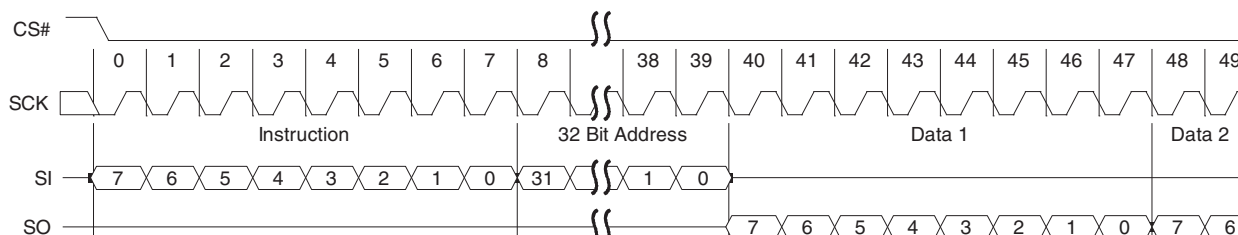
Figure 68 Fast Read Command Sequence (4-byte Address, 0Ch or 0B [ExtAdd=1], LC=11b)
