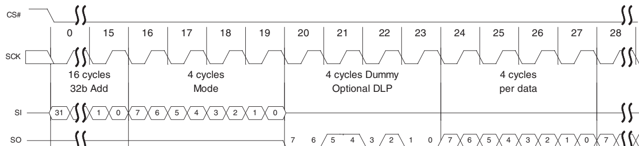
Figure 86 Continuous DDR Fast Read Subsequent Access (4-byte Address [ExtAdd=1], EHPLC=01b)
