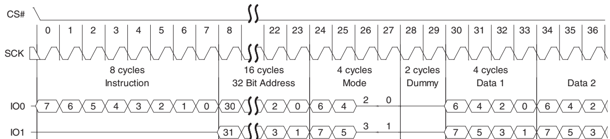
Figure 77 Dual I/O Read Command Sequence (4-byte Address, BCH or BBh [ExtAdd=1], EHPLC=10b)
