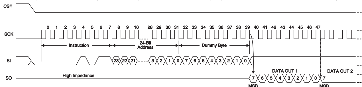
Figure 66 Fast Read (FAST_READ) Command Sequence (3-byte Address, 0Bh [ExtAdd=0, LC=10b])
