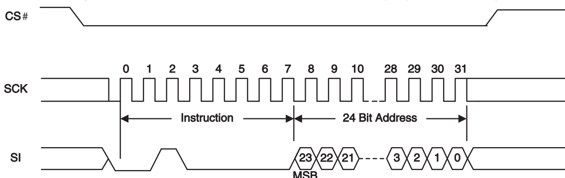
Figure 103 Parameter Sector Erase Command Sequence (3-Byte Address, 20h)
