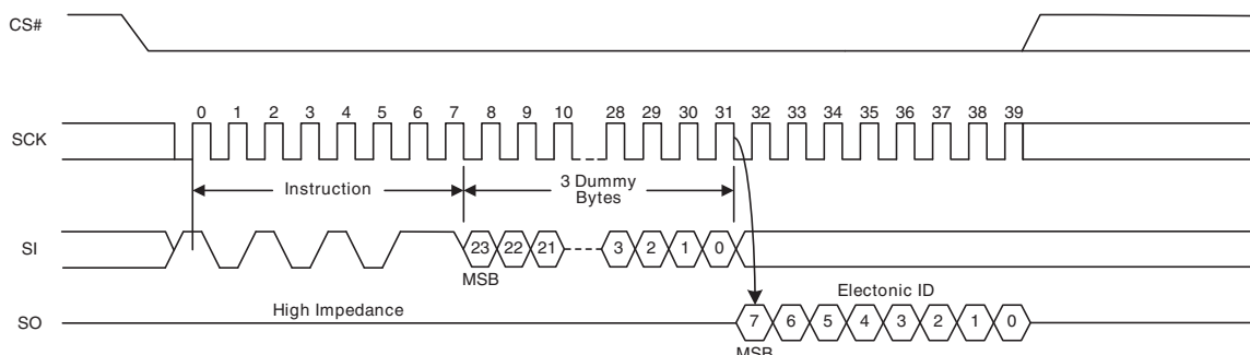
Figure 44 Read Electronic Signature (RES) Command Sequence
