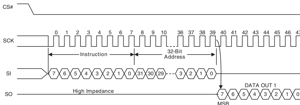
Figure 114 DYBRD Command Sequence
