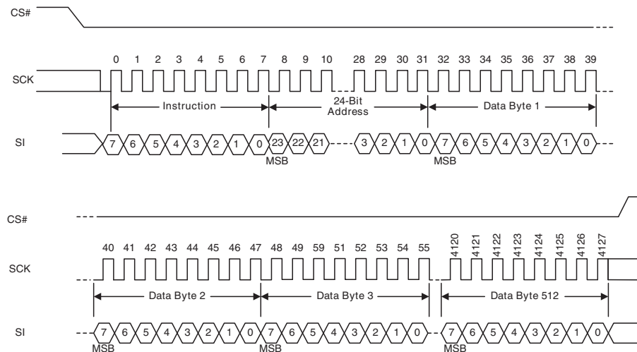
Figure 110 OTP Program Command Sequence
