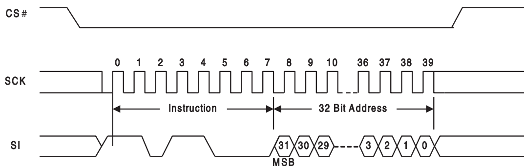
Figure 106 Sector Erase Command Sequence (ExtAdd = 1, D8h or 4-Byte Address, DCh)
