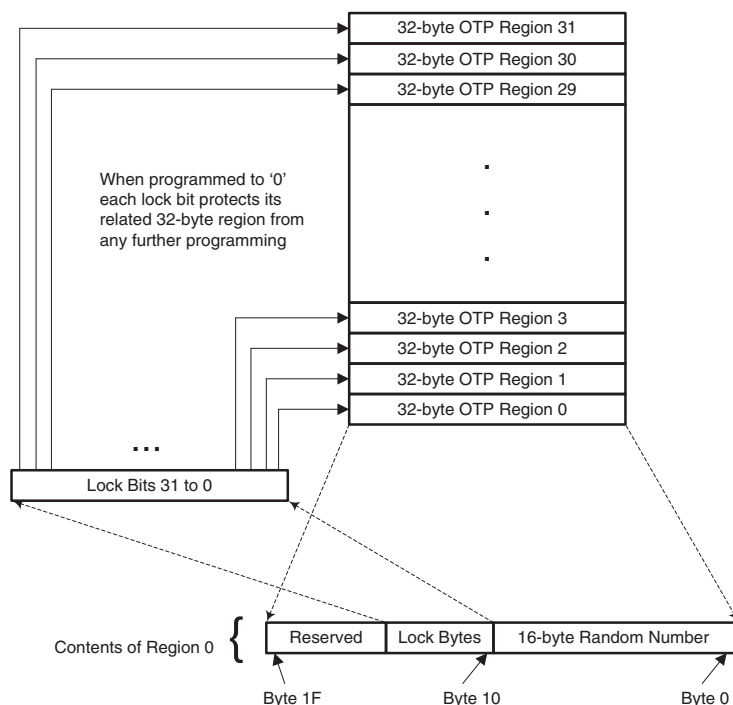
Figure 40 OTP Address Space
