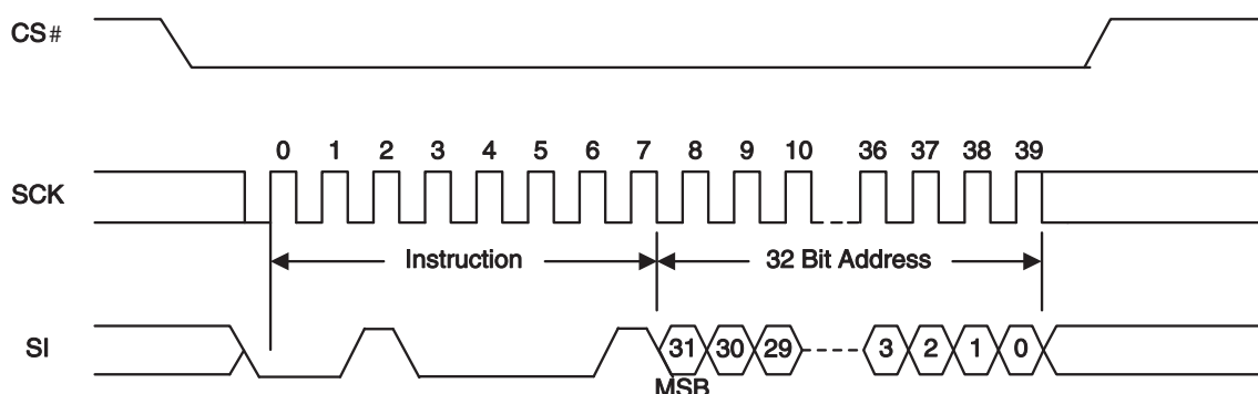
Figure 104 Parameter Sector Erase Command Sequence (ExtAdd = 1, 20h or 4-Byte Address, 21h)
