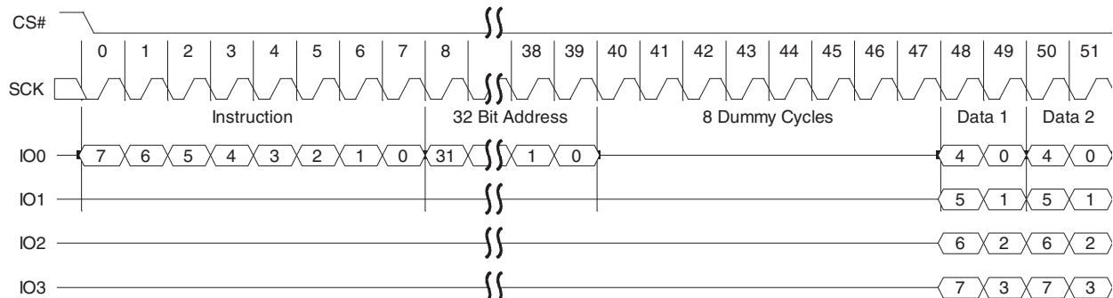
Figure 74 Quad Output Read Command Sequence (4-byte Address, 6Ch or 6Bh [ExtAdd=1], LC=11b)
