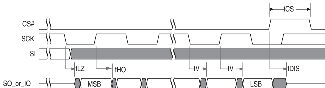
Figure 37 SPI DDR Output Timing
