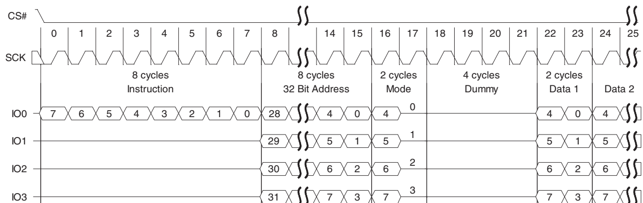
Figure 81 Quad I/O Read Command Sequence(4-byte Address, ECh or EBh [ExtAdd=1], LC=00b)
