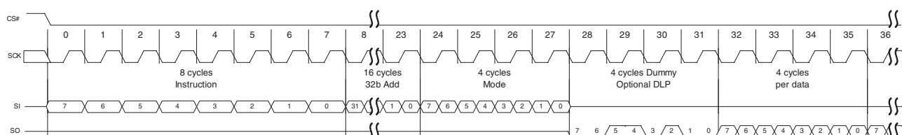
Figure 85 DDR Fast Read Initial Access (4-byte Address, 0Eh or 0Dh [ExtAdd=1], EHPLC=01b)
