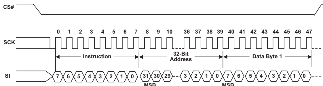
Figure 115 DYBWR Command Sequence
