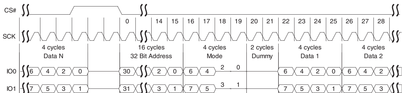
Figure 78 Continuous Dual I/O Read Command Sequence (4-byte Address, BCH or BBh [ExtAdd=1], EHPLC=10b)
