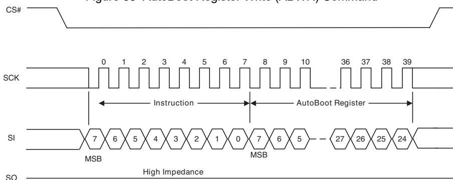
Figure 60 AutoBoot Register Write (ABWR) Command
