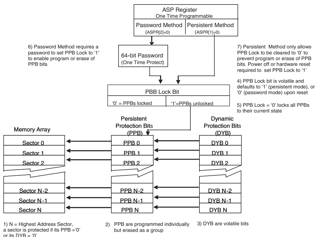
Figure 41 Advanced Sector Protection Overview
