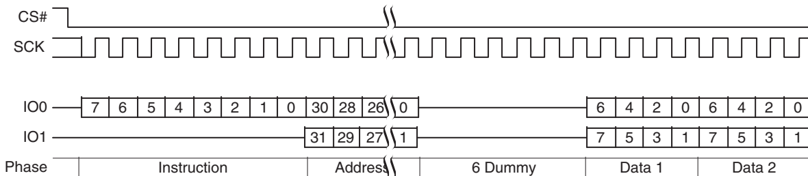
Figure 76 Dual I/O Read Command Sequence (4-byte Address, BBh [ExtAdd=1], HPLC=10b)
