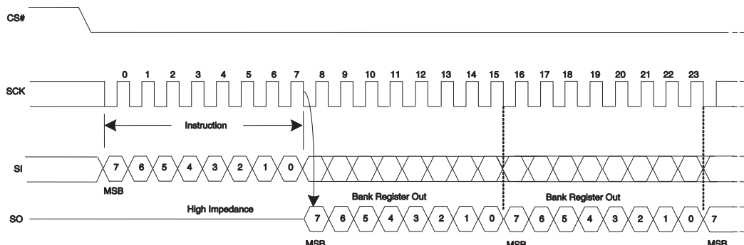
Figure 48 Read Bank Register (BRRD) Command
