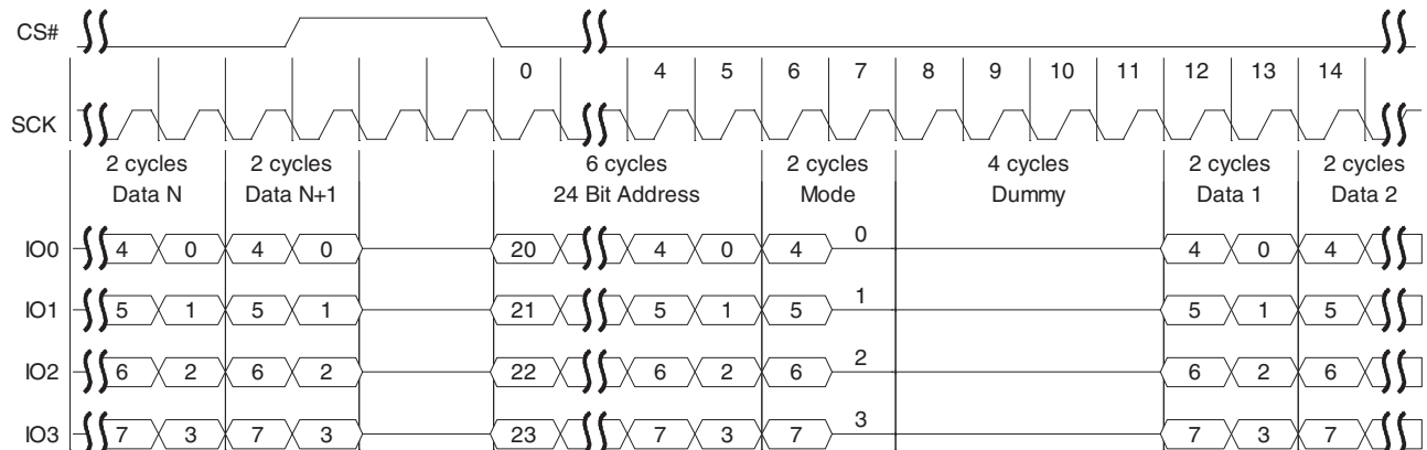
Figure 80 Continuous Quad I/O Read Command Sequence (3-byte Address), LC=00b
