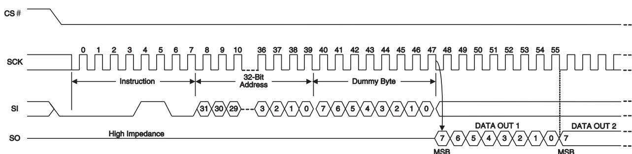
Figure 67 Fast Read Command Sequence (4-byte Address, 0Ch or 0B [ExtAdd=1], LC=10b)
