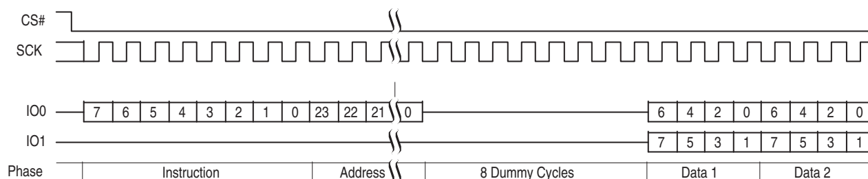
Figure 69 Dual Output Read Command Sequence (3-byte Address, 3Bh [ExtAdd=0], LC=10b)
