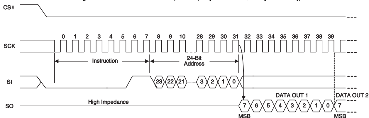
Figure 64 Read Command Sequence (3-byte Address, 03h [ExtAdd=0])
