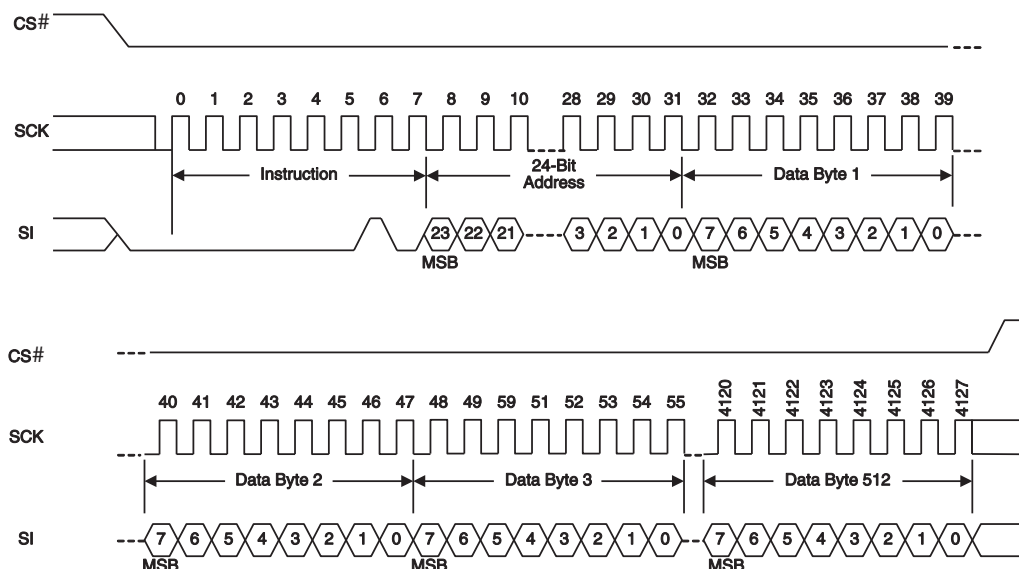
Figure 95 Page Program (PP) Command Sequence (3-byte Address, 02h)
