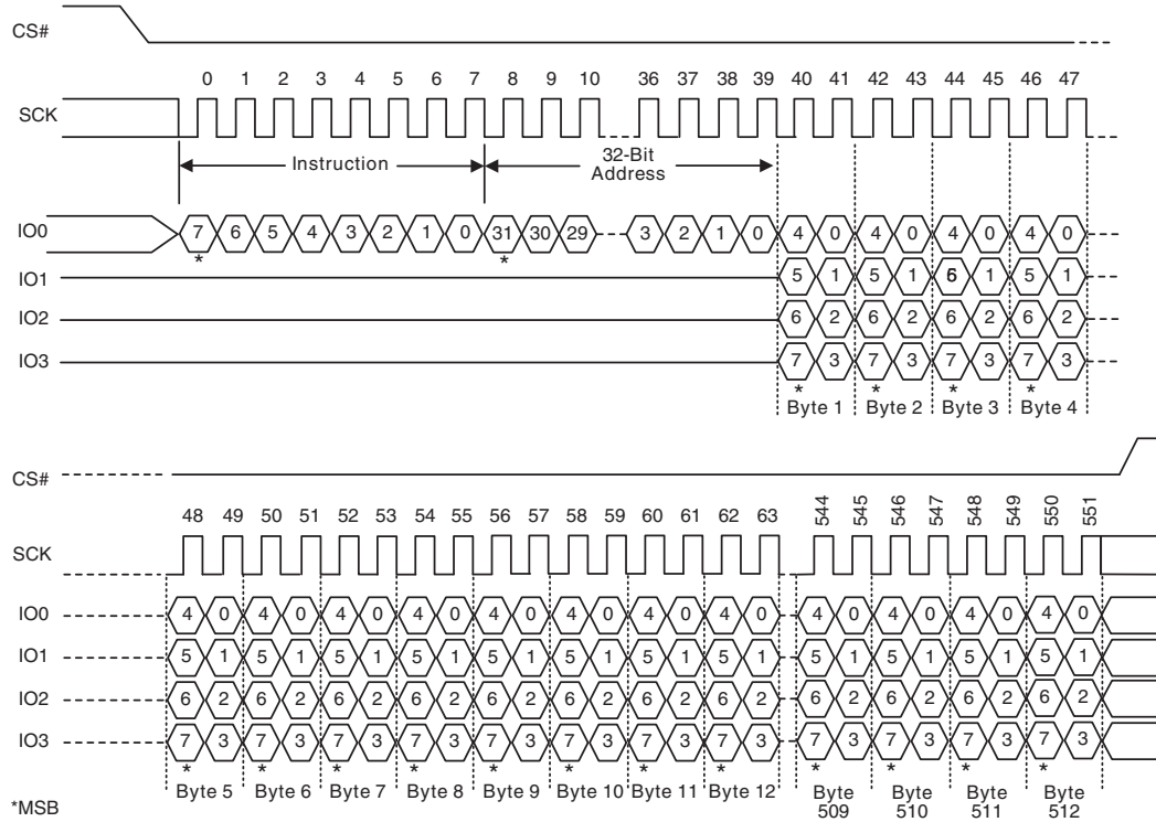
Figure 99 Quad 512-Byte Page Program Command Sequence (4-Byte Address, 34h or 32h or 38h [ExtAdd=1])
