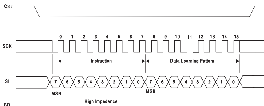
Figure 61 Program NVDLR (PNVDLR) Command Sequence
