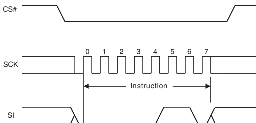
Figure 53 Write Enable (WREN) Command Sequence
