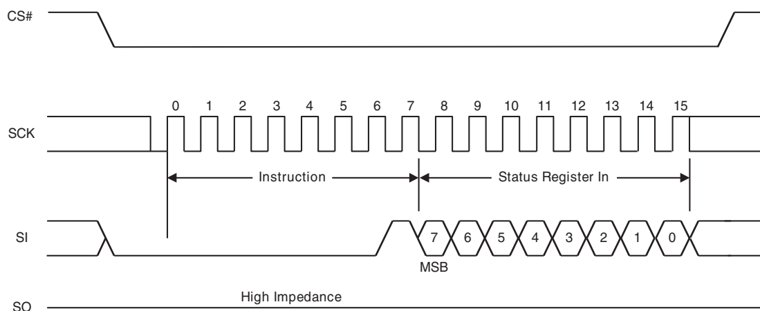
Figure 51 Write Registers (WRR) Command Sequence – 8 data bits
