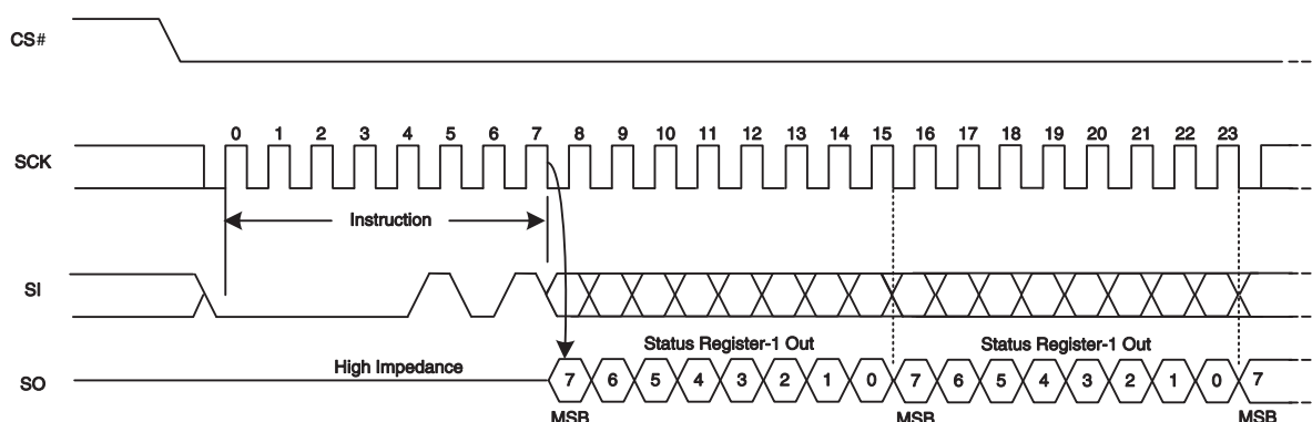
Figure 45 Read Status Register-1 (RDSR1) Command Sequence
