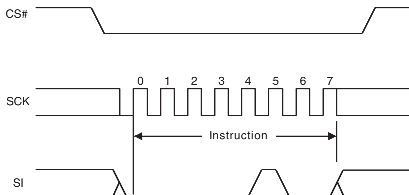
Figure 54 Write Disable (WRDI) Command Sequence
