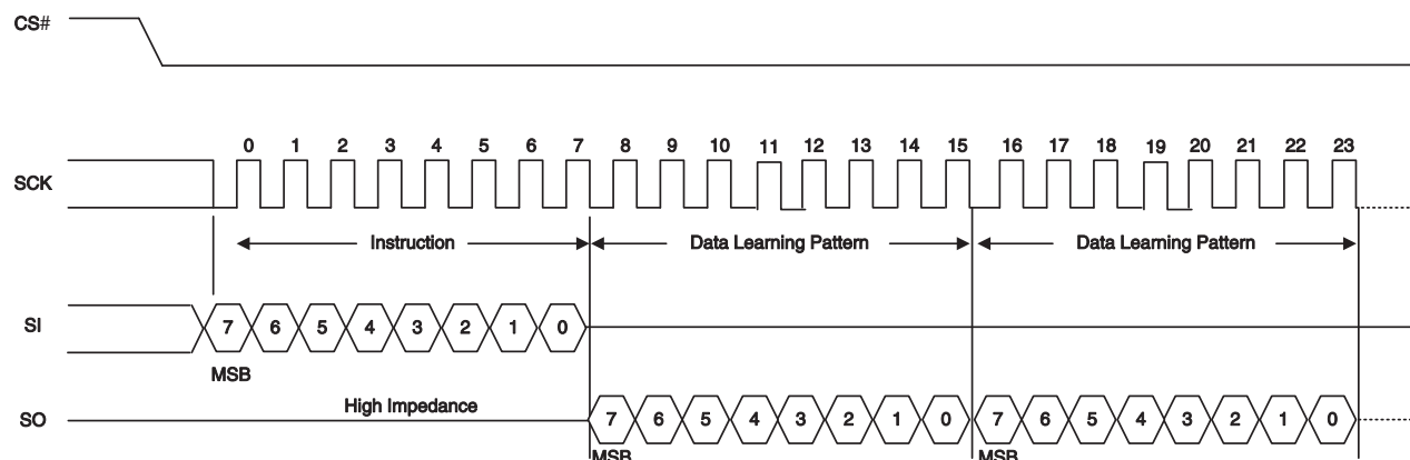
Figure 63 DLP Read (DLPRD) Command Sequence
