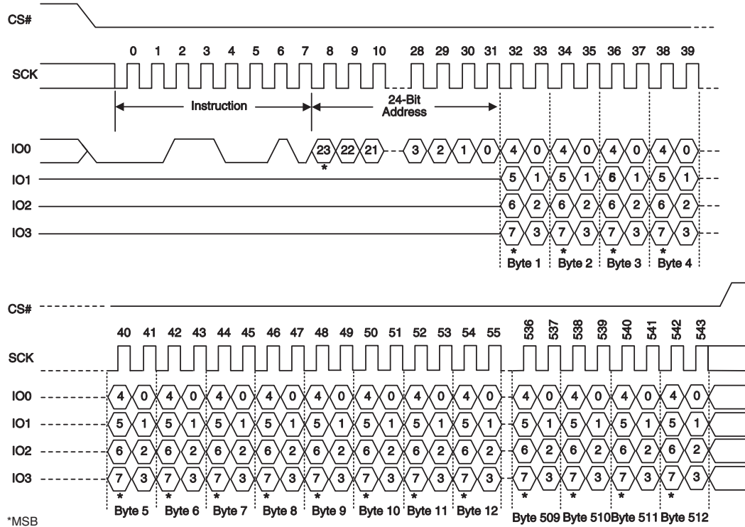
Figure 97 Quad 512-Byte Page Program Command Sequence (3-Byte Address, 32h or 38h)
