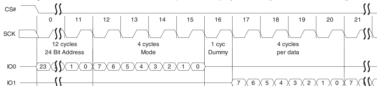
Figure 84 Continuous DDR Fast Read Subsequent Access (3-byte Address [ExtAdd=0, EHPLC=11b])
