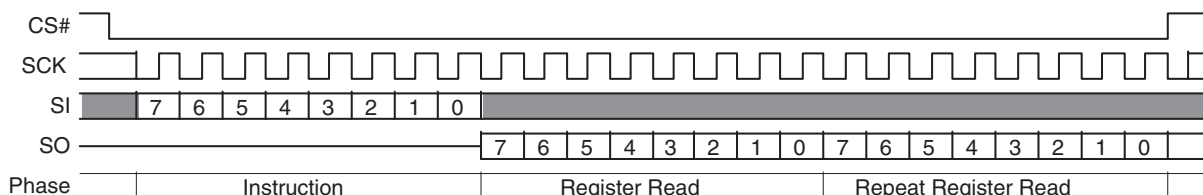
Figure 47 Read Configuration Register (RDCR) Command Sequence
