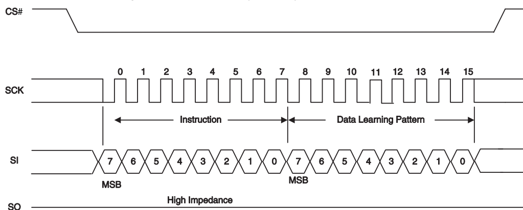
Figure 62 Write VDLR (WVDLR) Command Sequence
