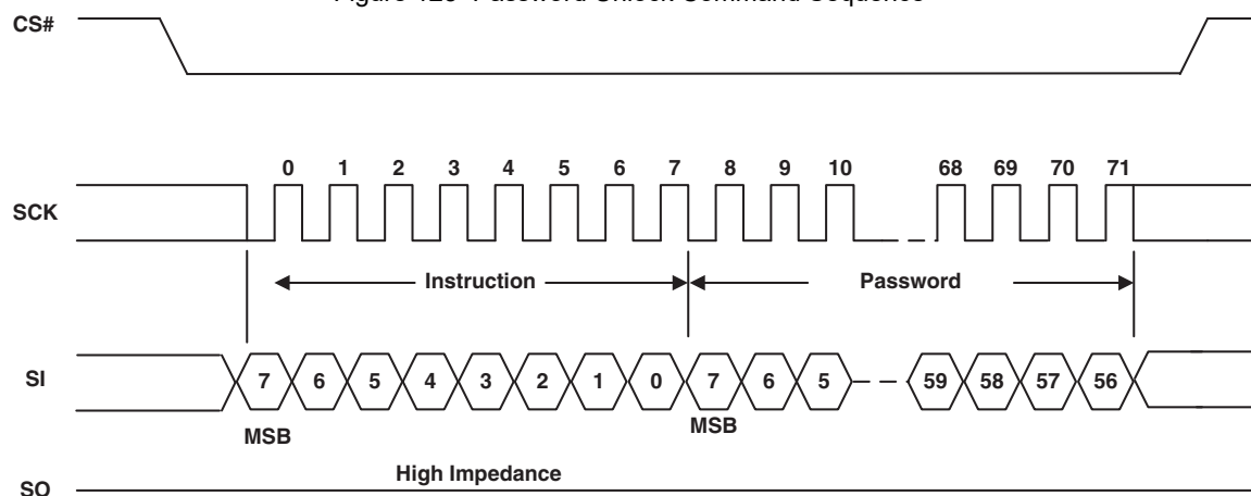
Figure 123 Password Unlock Command Sequence
