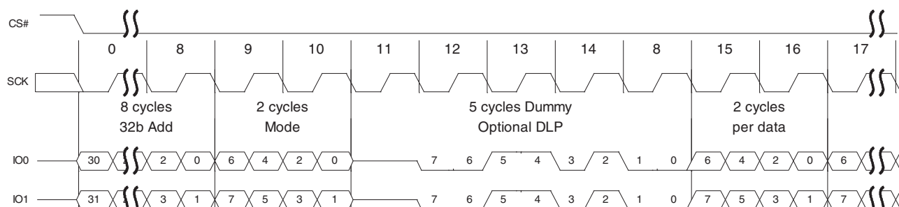
Figure 89 Continuous DDR Dual I/O Read Subsequent Access (4-byte Address, EHPLC= 01b)
