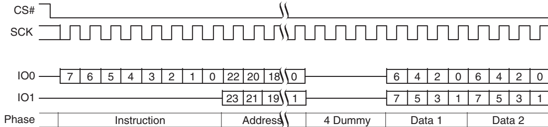
Figure 75 Dual I/O Read Command Sequence (3-byte Address, BBh [ExtAdd=0], HPLC=00b)
