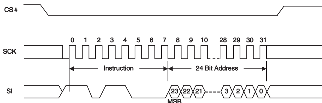
Figure 105 Sector Erase Command Sequence (ExtAdd = 0, 3-Byte Address, D8h)
