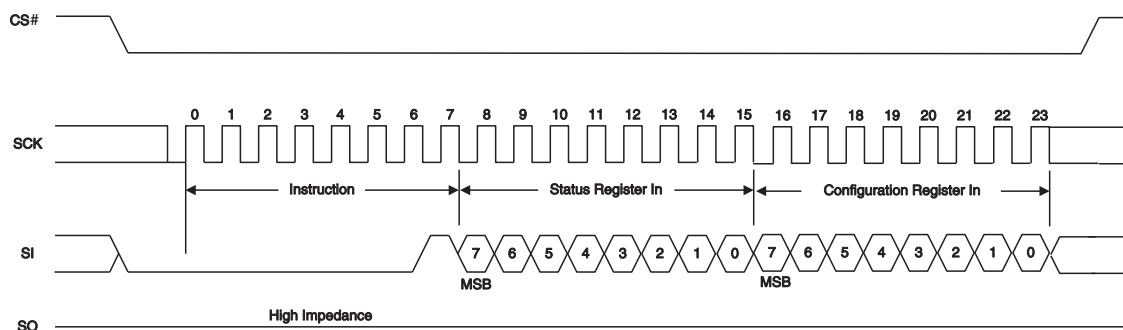
Figure 52 Write Registers (WRR) Command Sequence – 16 data bits
