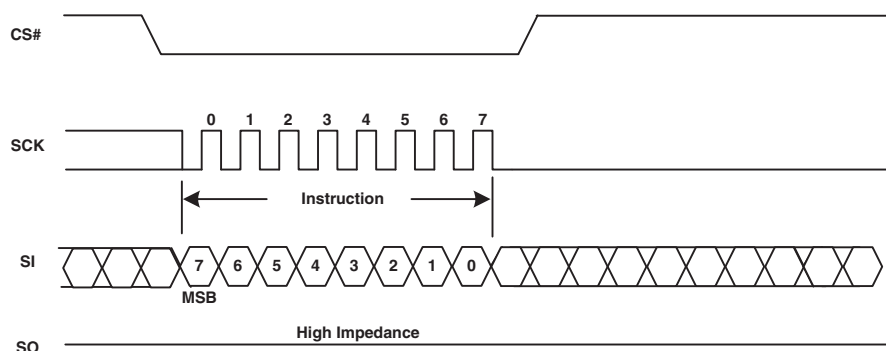
Figure 50 BRAC (B9h) Command Sequence
