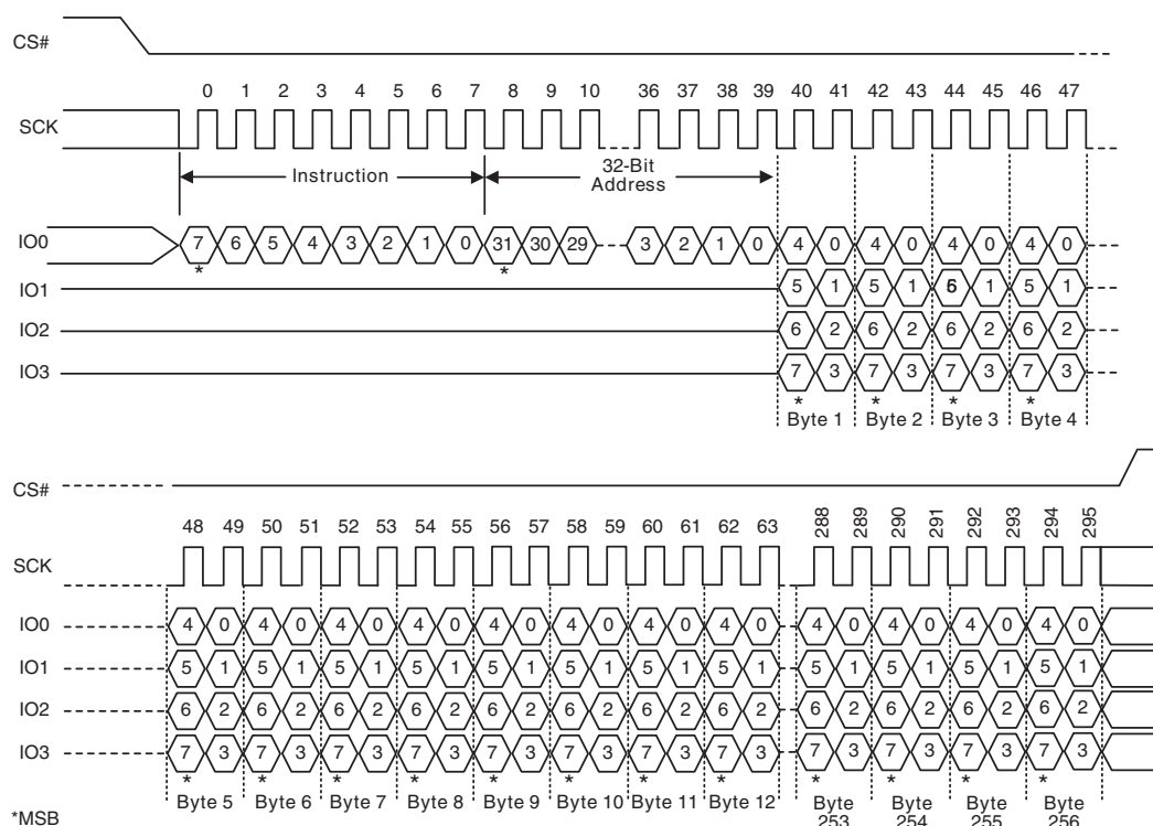
Figure 100 Quad 256-Byte Page Program Command Sequence (4-Byte Address, 34h or 32h or 38h [ExtAdd=1])
