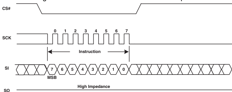
Figure 120 PPB Lock Bit Write Command Sequence
