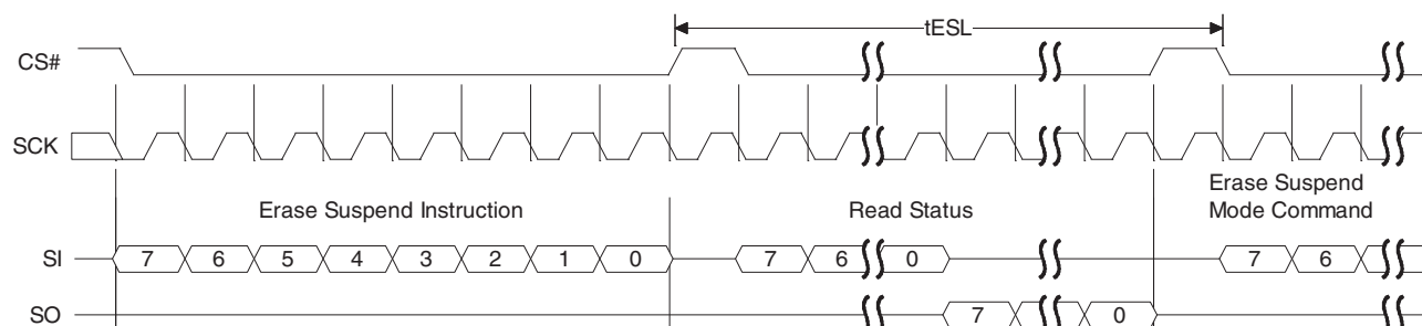
Figure 108 Erase Suspend Command Sequence
