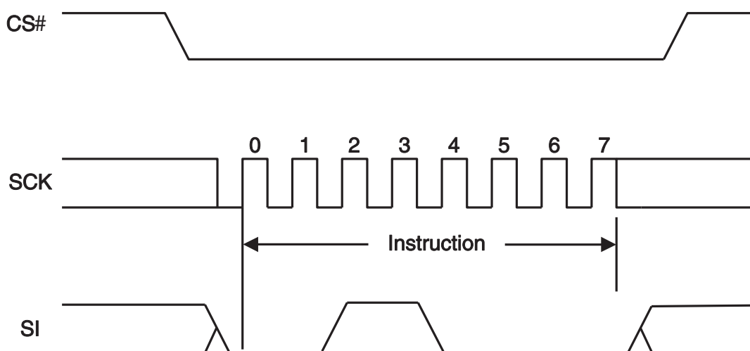
Figure 55 Clear Status Register (CLSR) Command Sequence
