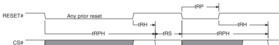
Figure 29 Hardware Reset
