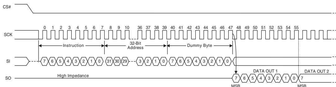
Figure 56 ECC Status Register Read Command Sequence
