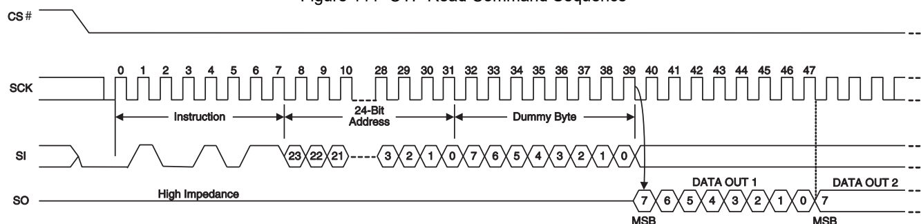
Figure 111 OTP Read Command Sequence
