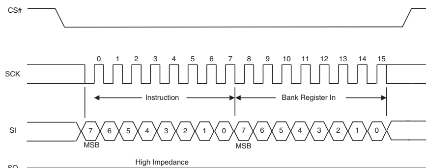
Figure 49 Bank Register Write (BRWR) Command
