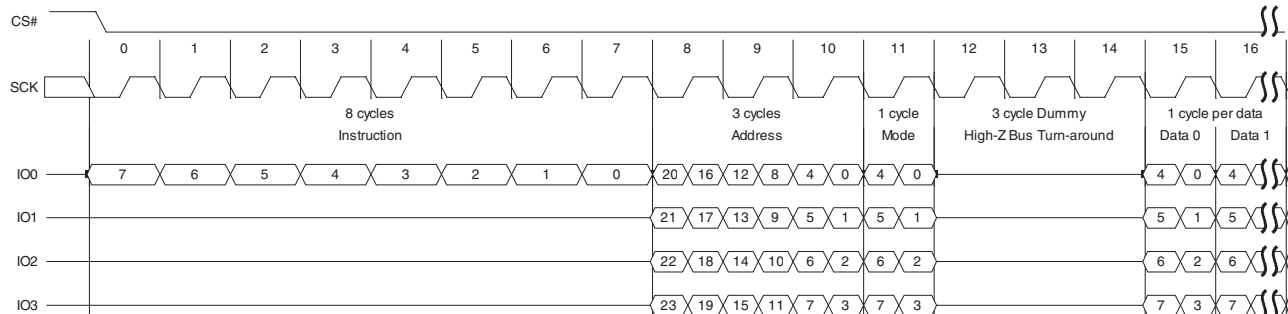
Figure 91 DDR Quad I/O Read Initial Access (3-byte Address, EDh [ExtAdd=0], HPLC=11b)
