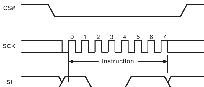
Figure 107 Bulk Erase Command Sequence
