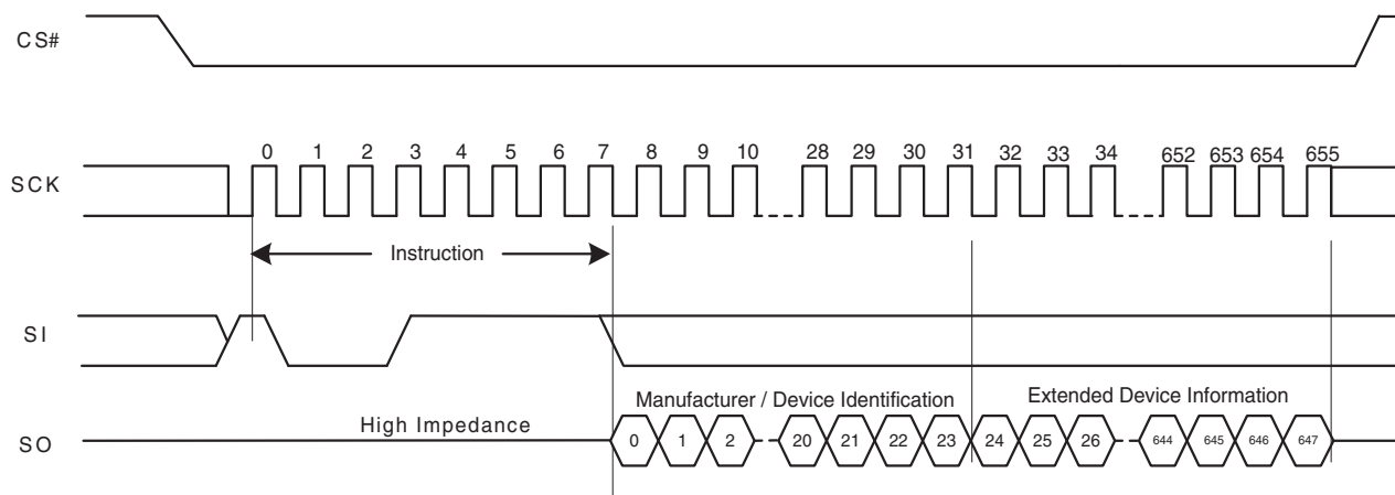
Figure 43 Read Identification (RDID) Command Sequence
