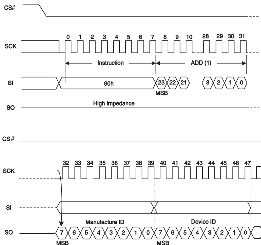
Figure 42 READ_ID Command Sequence
