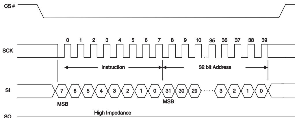
Figure 117 PPBP Command Sequence
