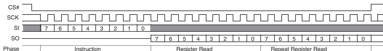
Figure 119 PPB Lock Register Read Command Sequence
