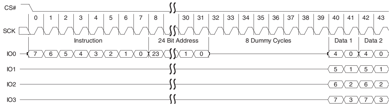
Figure 72 Quad Output Read Command Sequence (3-byte Address, 6Bh [ExtAdd=0, LC=01b])
