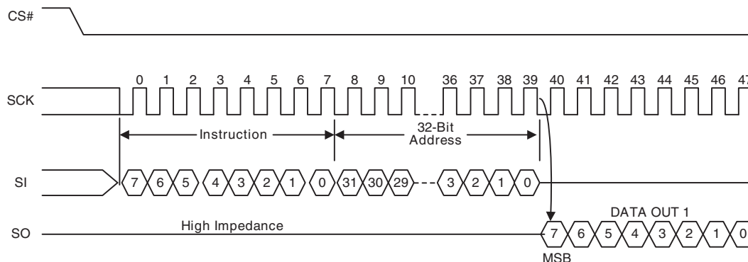
Figure 116 PPBRD Command Sequence
