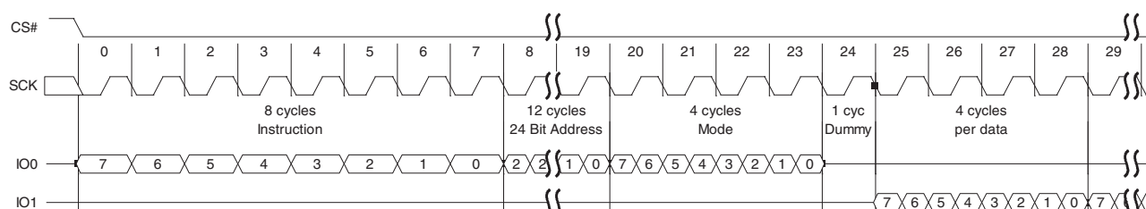
Figure 83 DDR Fast Read Initial Access (3-byte Address, 0Dh [ExtAdd=0, EHPLC=11b])
