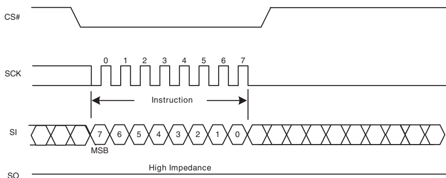
Figure 118 PPB Erase Command Sequence
