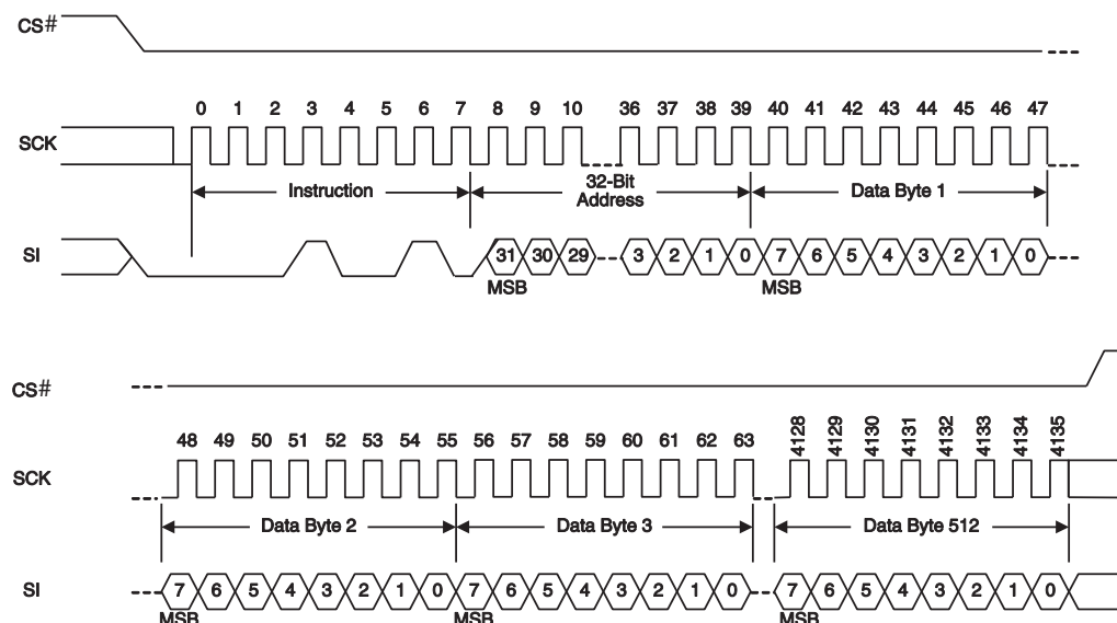
Figure 96 Page Program (4PP) Command Sequence (4-byte Address, 12h)
