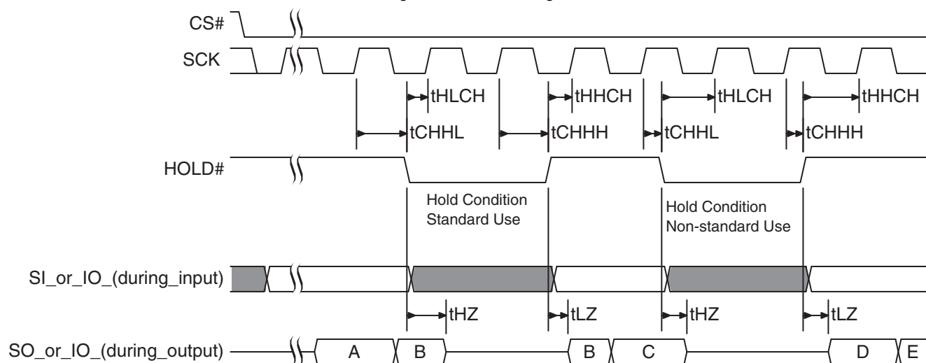
Figure 34 Hold Timing
