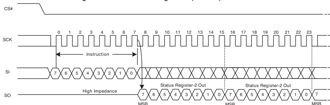
Figure 46 Read Status Register-2 (RDSR2) Command
