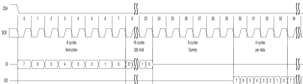
Figure 87 DDR Fast Read Subsequent Access (4-byte Address, HPLC=01b)
