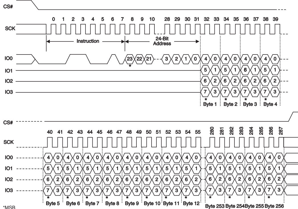
Figure 98 Quad 256-Byte Page Program Command Sequence (3-Byte Address, 32h or 38h)
