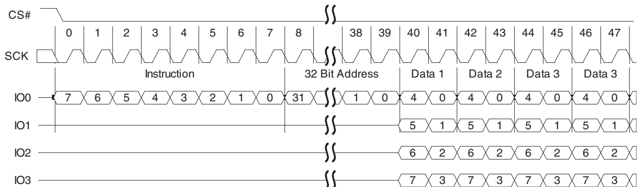
Figure 74 Quad Output Read Command Sequence (4-byte Address, 6Ch or 6Bh [ExtAdd=1], LC=11b)
