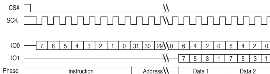
Figure 71 Dual Output Read Command Sequence (4-byte Address, 3Ch or 3Bh [ExtAdd=1, LC=11b])
