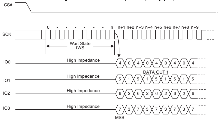
Figure 58 AutoBoot Sequence (CR1[1]=1)
