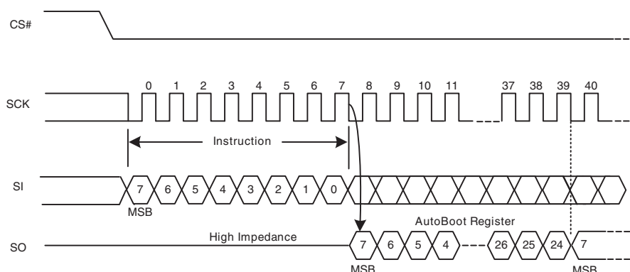
Figure 59 AutoBoot Register Read (ABRD) Command
