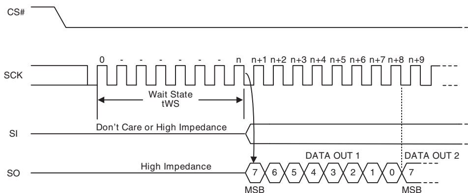
Figure 57 AutoBoot Sequence (CR1[1]=0)
