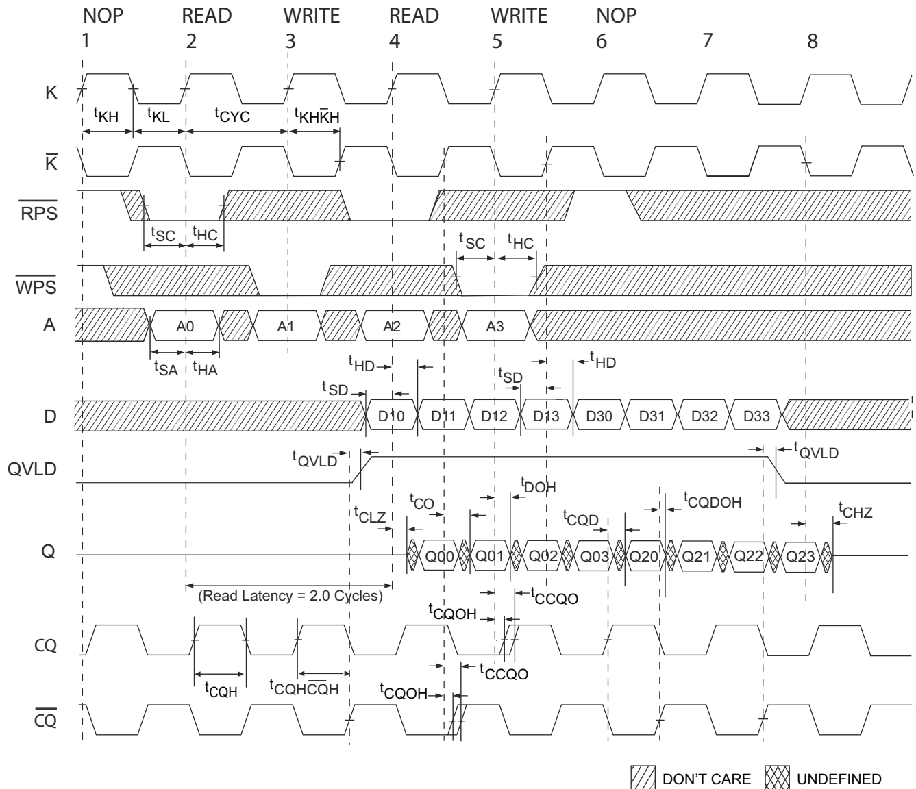
Figure 5. Waveform for 2.0 Cycle Read Latency [31, 32, 33]
