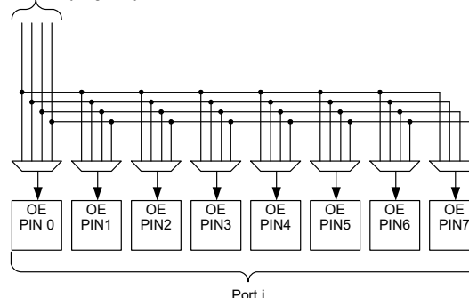
Figure 7-13. I/O Pin Output Enable Connectivity
