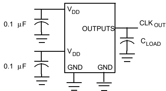
Figure 3. Test Circuit # 1
