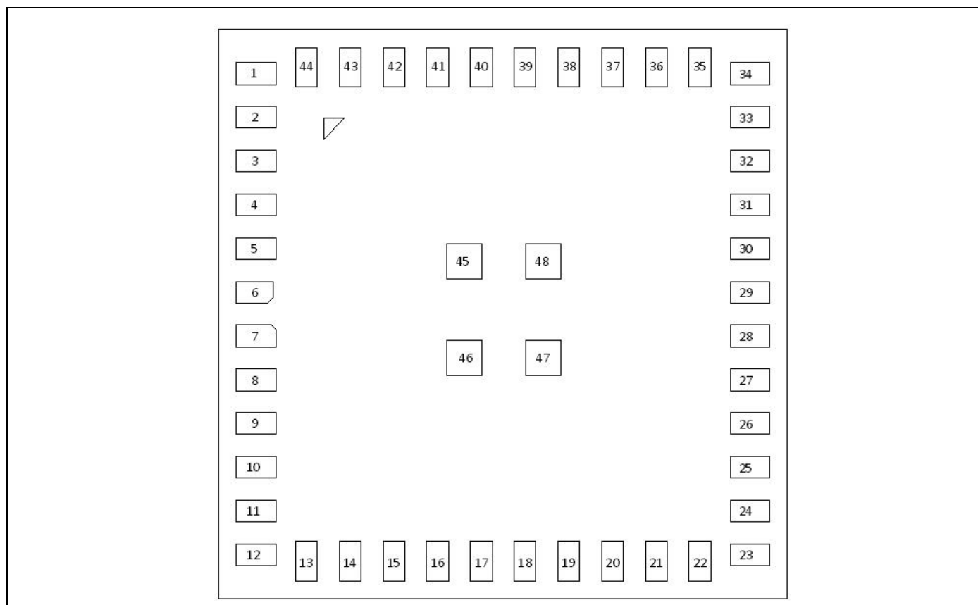
Figure 3. CYW20737S (TOP View)
