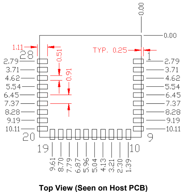
Figure 6. CYBT-4230xx-02 Host Layout (Relative to Origin)
