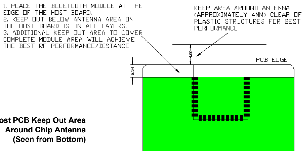
Figure 4. Optional Additional Host PCB Keep Out Area Around the CYBT-4230xx-02 Chip Antenna
