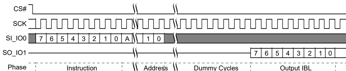
Figure 95. IBLRD Command Sequence [52, 53]
