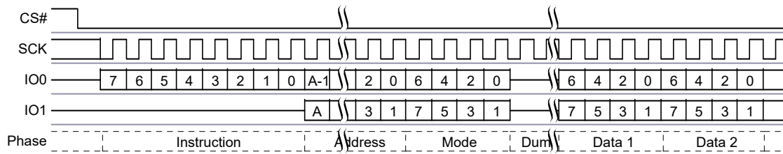
Figure 70. Dual I/O Continuous Read Command Sequence [34]
