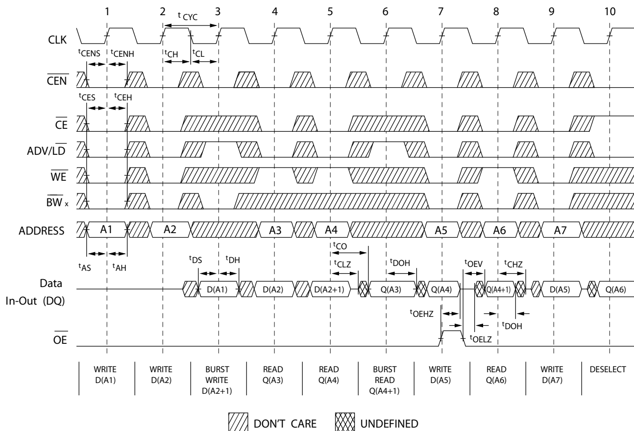
Figure 6. Read/Write Timing [26, 27, 28]
