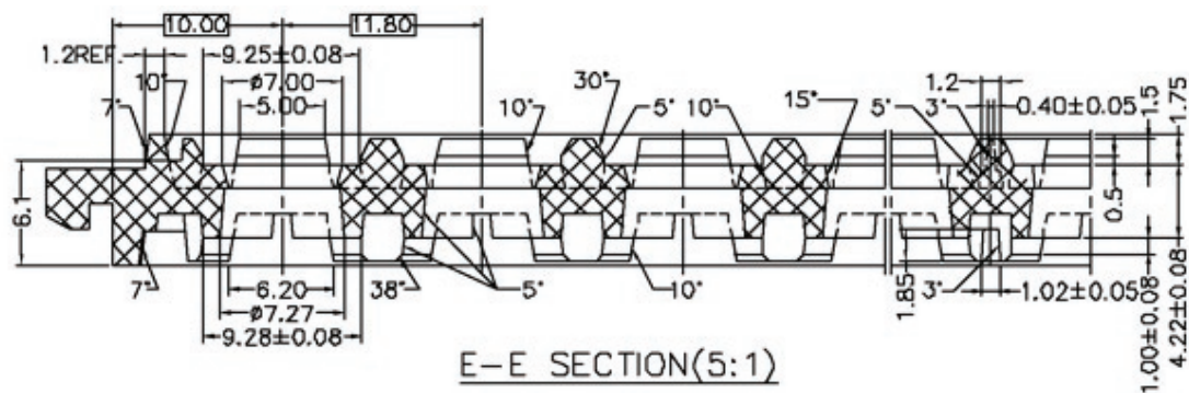
Figure 35. CYW20733 9 × 9 FBGA Package Tray (2 of 2)
