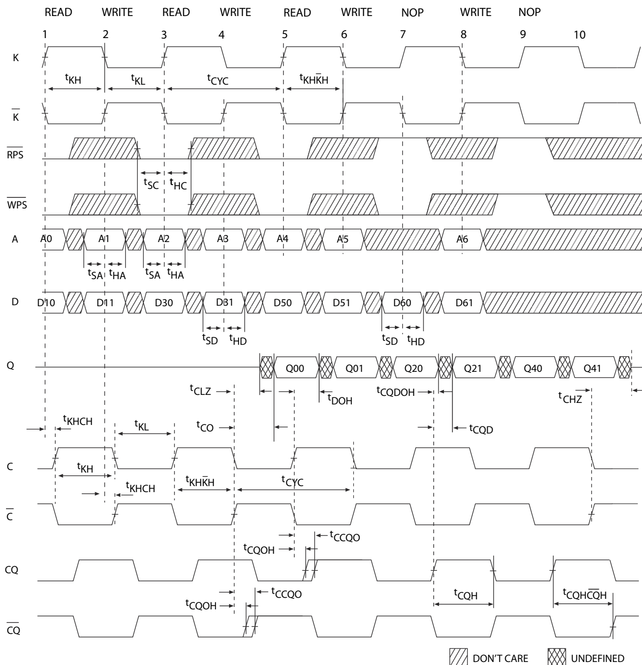
Figure 6. Read/Write/Deselect Sequence [35, 36, 37]
