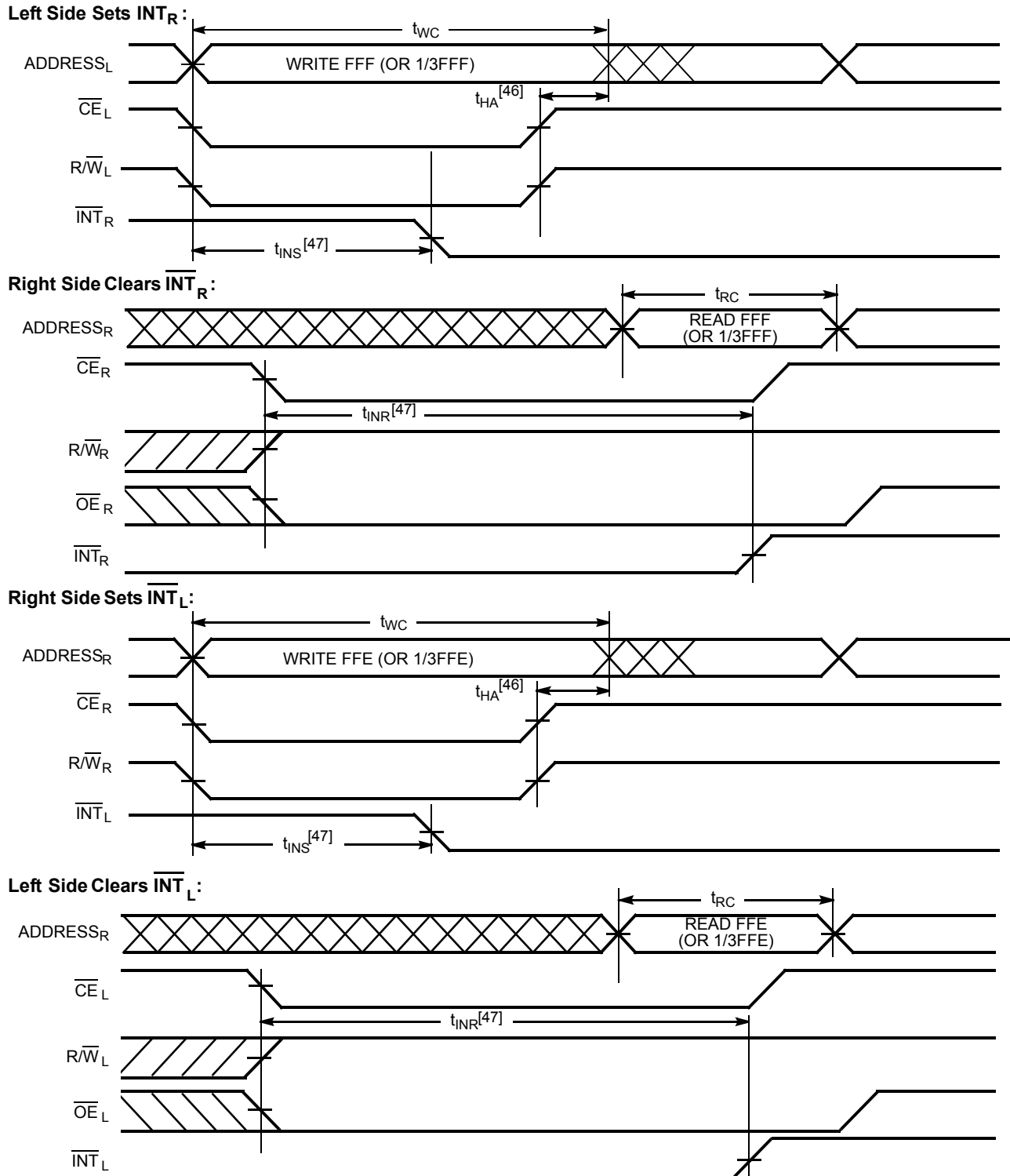
Figure 15. Interrupt Timing Diagram
