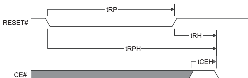
Figure 16.4 Hardware Reset
