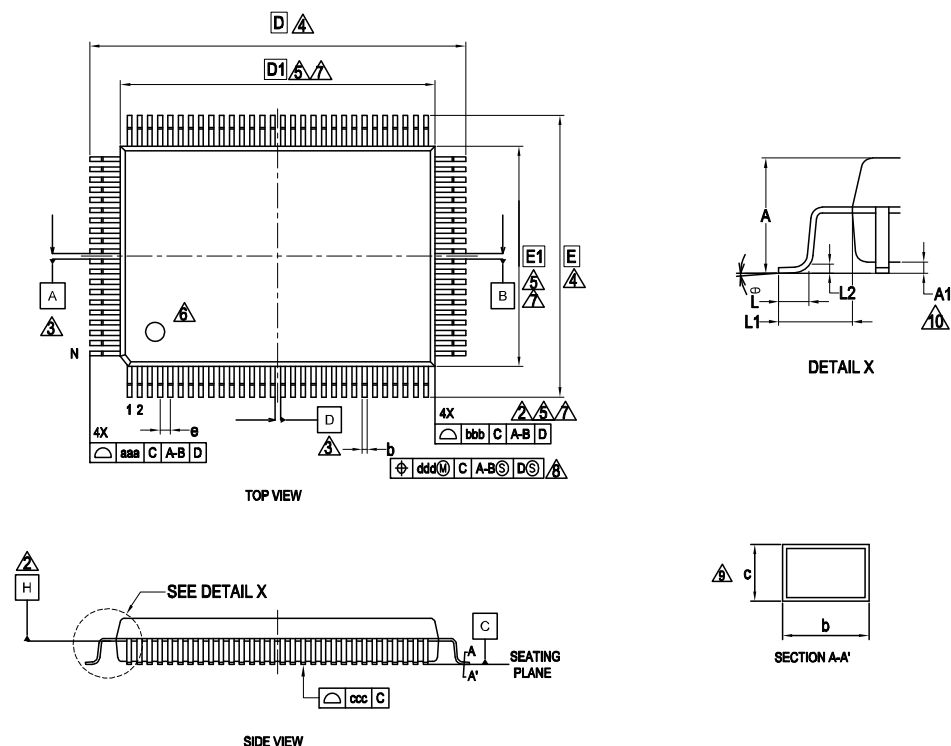
PQH100 , 100 Lead Plastic Quad Flat Package
