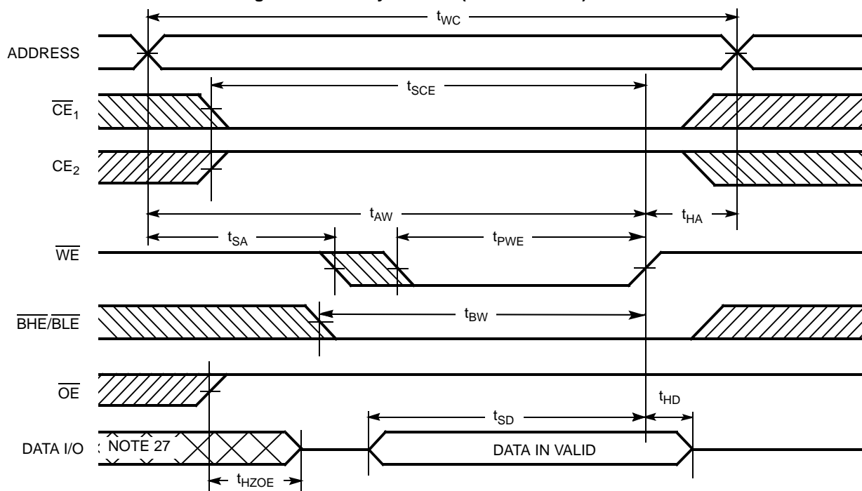
Figure 7. Write Cycle No. 2 ( \overline{\text{CE}}_1 or \overline{\text{CE}}_2 Controlled) [24, 25, 26]
