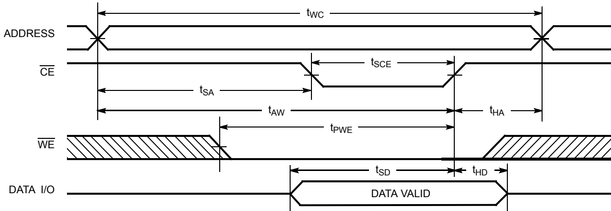
Figure 7. Write Cycle No. 2 ( \overline{\text{CE}} Controlled) [27, 28]
