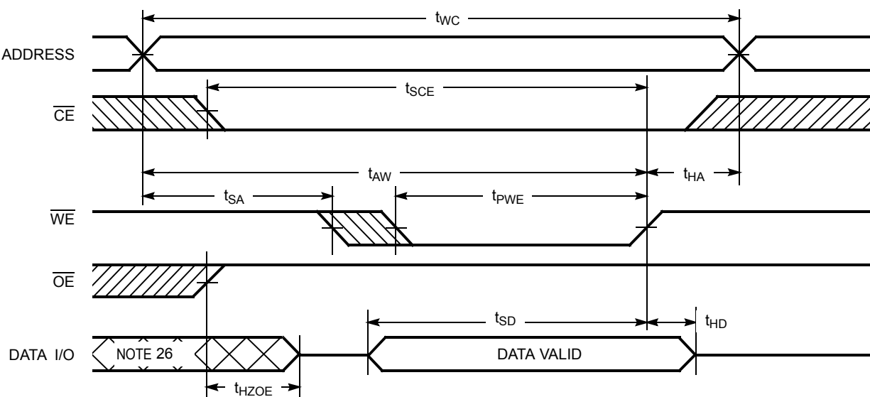
Figure 6. Write Cycle No. 1 ( \overline{\text{WE}} Controlled, \overline{\text{OE}} HIGH During Write) [24, 25]
