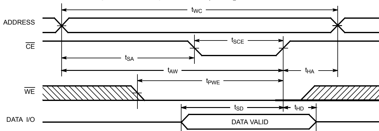
Figure 11. Write Cycle No. 3 ( \overline{WE} Controlled, \overline{OE} LOW) [27, 30]
