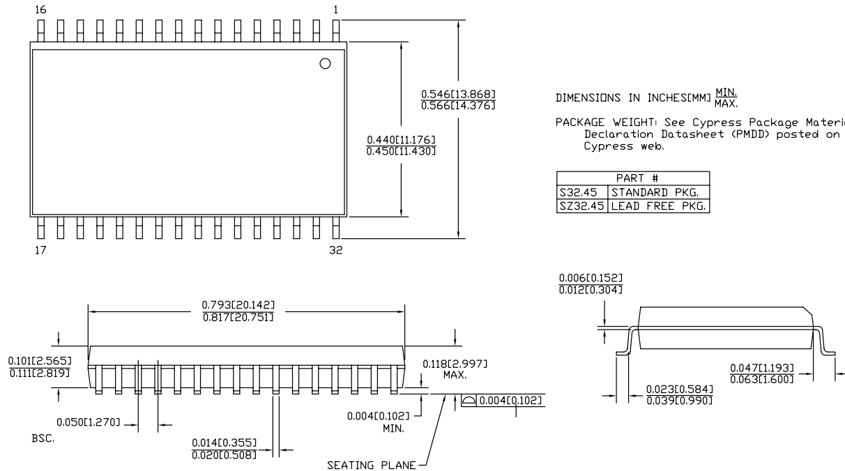
Figure 14. 32-pin Molded SOIC (450 Mil) S32.45/SZ32.45, 51-85081
