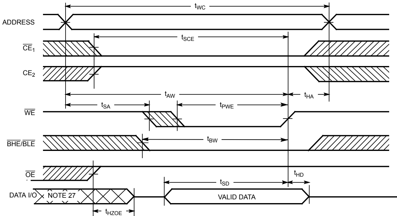
Figure 7. Write Cycle No. 1 ( \overline{\text{WE}} Controlled) [24, 25, 26]
