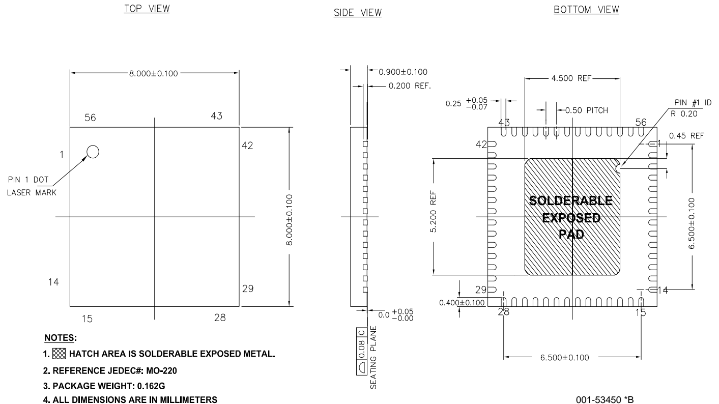
Figure 4. 56-pin QFN (8 × 8 × 0.9 mm) - Sawn
