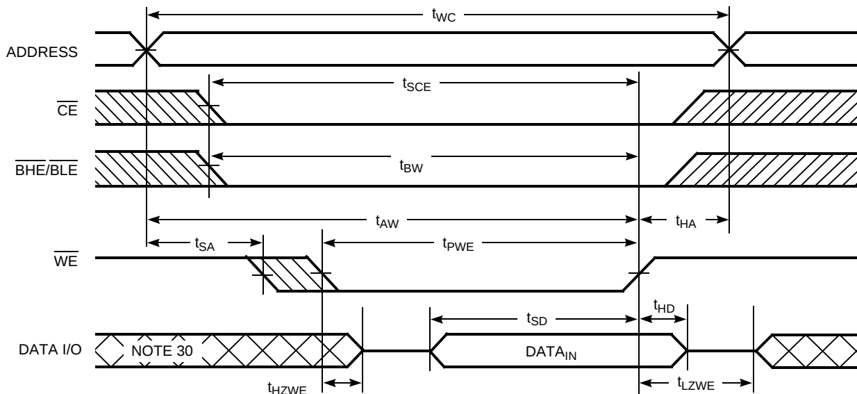
Figure 9. Write Cycle No. 4 ( \overline{\text{BHE/BLER}} Controlled, \overline{\text{OE}} LOW) [28, 29]
