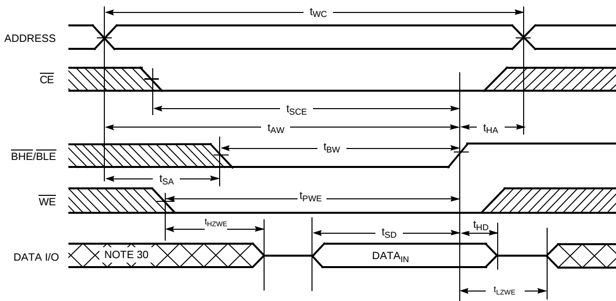
Figure 9. Write Cycle No. 4 ( \overline{\text{BHE/BLER}} Controlled, \overline{\text{OE}} LOW) [28, 29]
